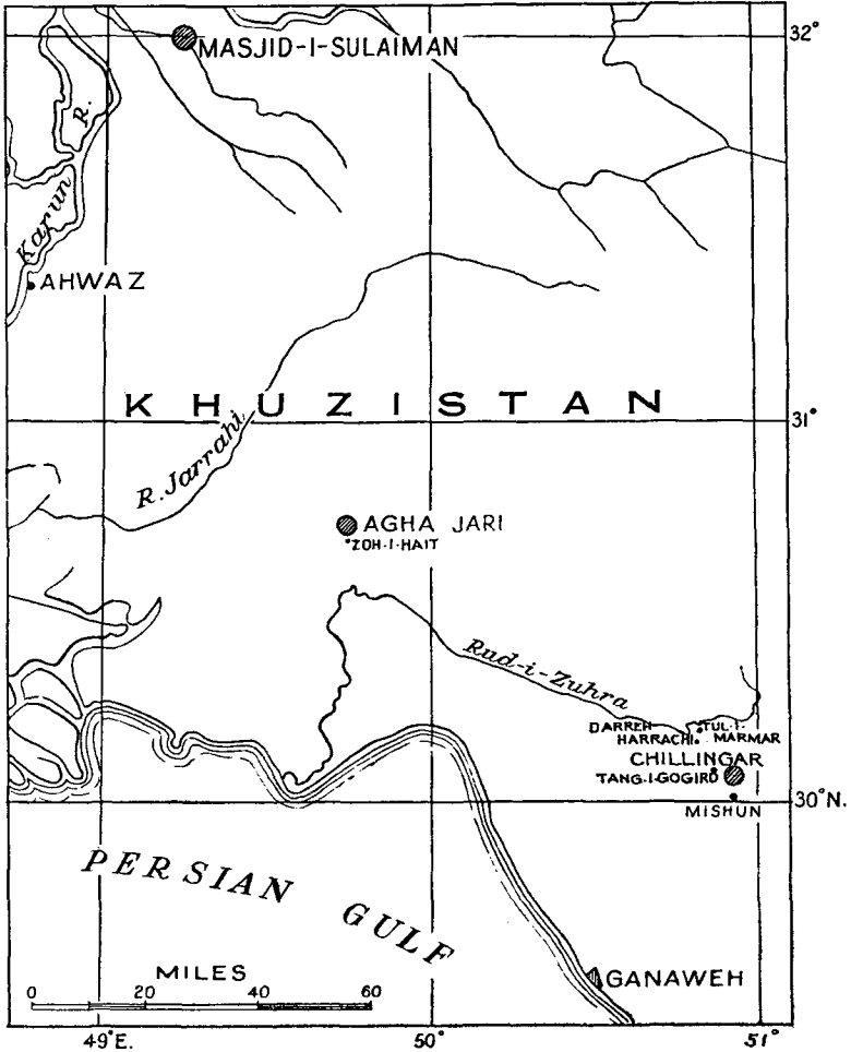
FIG. 1. Sketch-map showing localities referred to in the text.
