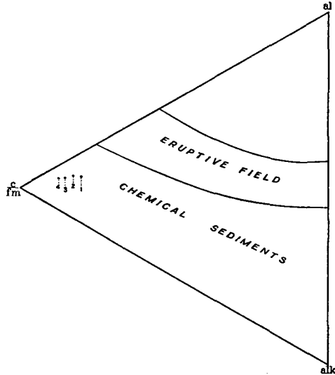
FIG. 3. Diagram showing the relation of the analysed rocks to known eruptive types.
