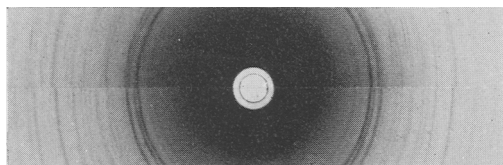
FIG. 4 ( upper ). X-ray photograph of tacharanite, Portree, Isle of Skye, 6 cm.-diam. camera (B.M. 1961, 163). ( lower ). X-ray photograph of type tobermorite, Tobermory, Isle of Mull, 6-cm. diam. camera (Heddle collection, Royal Scottish Museum, S.M.C. 435A1, X-ray No. 5418).
