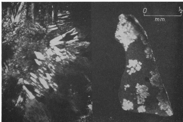
FIG. 2 ( left ). Acicular mesolite terminating in birefringent paddle-shaped crystals penetrating tobermorite, Portree, Isle of Skye. Crossed nicols, \times 44 (B.M. 1961, 162). FIG. 3 ( right ). Tacharanite, almost isotropic, with inclusions of birefringent gyrolite, fragment, Portree, Isle of Skye. Crossed nicols, \times 50 (B.M. 1961, 163).
