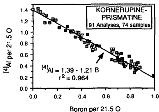
FIG. 1. Plot of 91 kornerupine (here sensu stricto ) and prismatine compositions obtained on 74 samples in terms of boron and ^{[4]}\text{Al} (calculated from 5 - Si - B - Be) per formula unit of 21.5 oxygens. Sources of data are Table 2; Grew et al. (1987, 1990); Friend, 1995; Cooper and Hawthorne, unpublished data; and the literature cited in Grew (in prep.).
