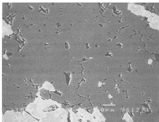
FIG. 1. Back-scattered electron image of okayamalite (grey) and vesuvianite (white to light grey). Bar indicates 10 \mu\text{m} .
