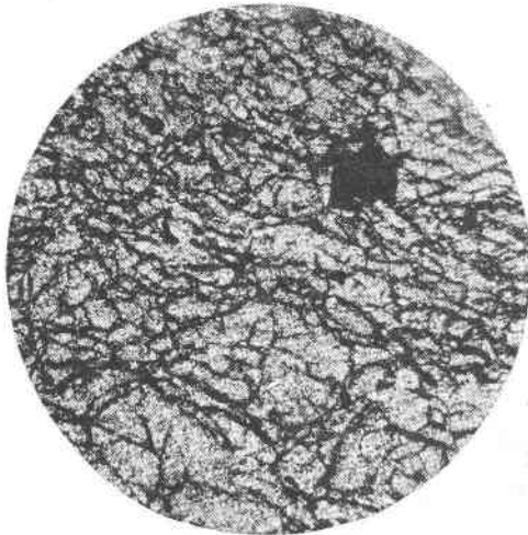
FIG. 1. Highly magnified photograph by transmitted light of a thin section of Sabine township euxenite, showing regular fracturing and freedom from inclusions. The black spot represents a hole in the section. The photograph does not give a true picture of the section. Actually the fractures are very narrow and sharp with little or no alteration along the edges.
