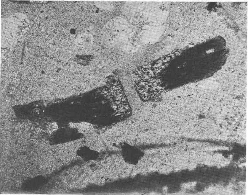
FIG. 12. Two biotite crystals resorbed to a dust of iron oxide, pyroxene, etc., in the central part of the figure but fresh except for a little iron stain to the right and left. Fisher latite-andesite, northern part of San Cristobal quadrangle, west of Lake San Cristobal on ridge south of Grassy Mountain, at an elevation of 11,400 feet. 45X.
