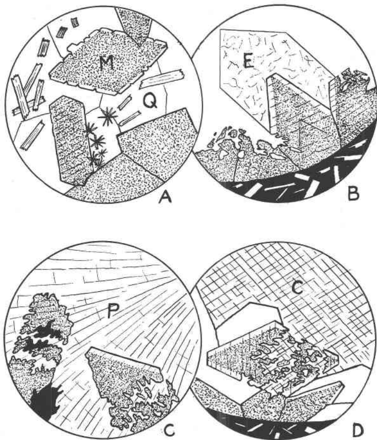
FIG. 2. Some features of the paragenesis seen in thin sections. Magnification about 25X
