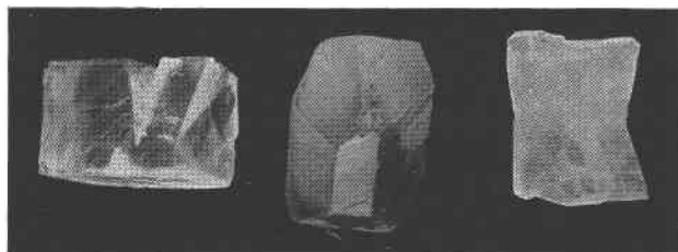
FIG. 3. (01\bar{1}2) twins in calcite; left: "knife blade" twin similar to those illustrated in Figs. 1 and 2. Center: twin-gliding lamellae on a crystal of calcite from Egremont, England. The crystal is bounded by cleavage rhombohedrons and prism faces. Compare with the projection Fig. 4. Right: growth twin from Guanajuato, Mexico.
