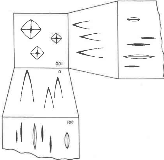
FIG. 4. Etch figures and hillocks on \{001\} , \{100\} and \{101\} of paramelaconite. Produced in 8 hours by \text{NH}_4\text{Cl} + \text{H}_2\text{SO}_4 solution. The absolute and relative sizes of the figures are greatly exaggerated.
