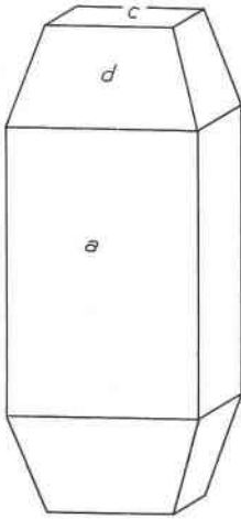
FIG. 2. Idealized crystal.
