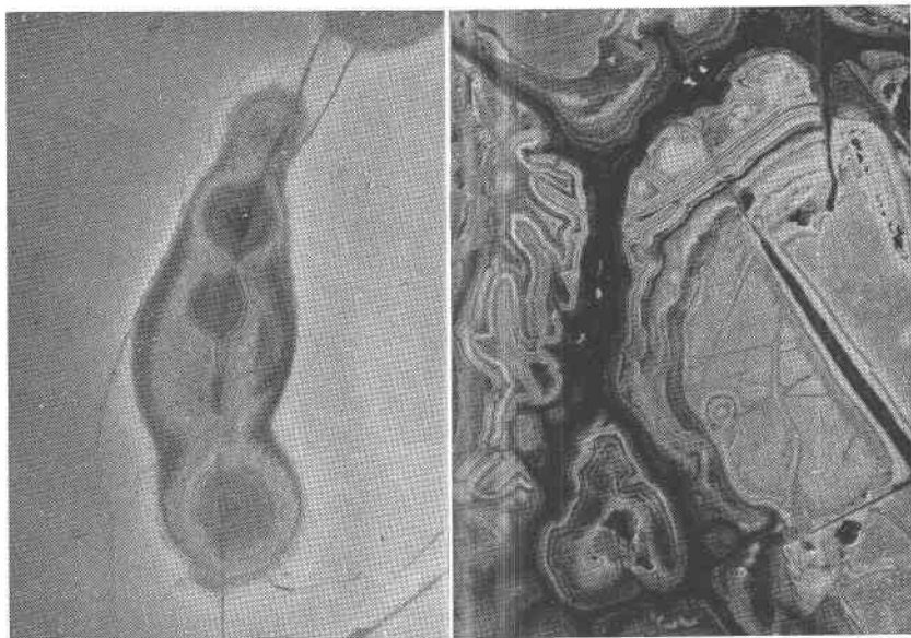
FIG. 2. Photograph showing small wardite-millsite spherules cut by a very thin veinlet of pseudowavellite and surrounded by pseudowavellite. The bands of the spherules tongue out when they meet the thin veinlet. \times 2 .
