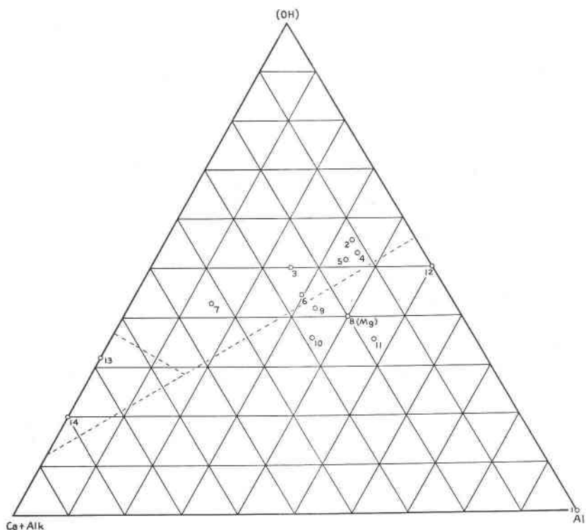
FIG. 5. Ternary diagram on which is plotted the atomic ratios Ca+alkalies:Al:OH of the analyzed minerals from the nodules. 1 variscite, 2 pseudowavellite, 3 deltaite, 4 millisite, 5 wardite, 6 lehiite, 7 dennisonite, 8 gordonite, 9 englishite, 10 montgomeryite, 11 overite, 12 sterrettite, 13 lewistonite, 14 dehrnite.
