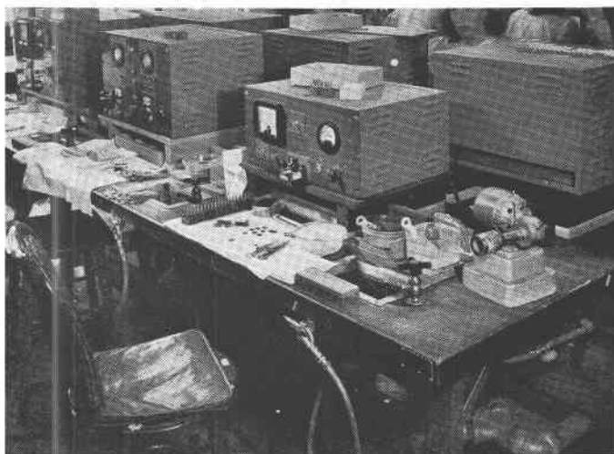
FIG. 8. Final etch finishing position. Note plastic tongs for immersing crystal in Pyrex bowl of etch solution, toothbrush and bowl of soap solution for cleaning, air gun, bowl of dilute ammonia water, comparison oscillator, and abrasive lined cylinder for beveling crystal edges.
