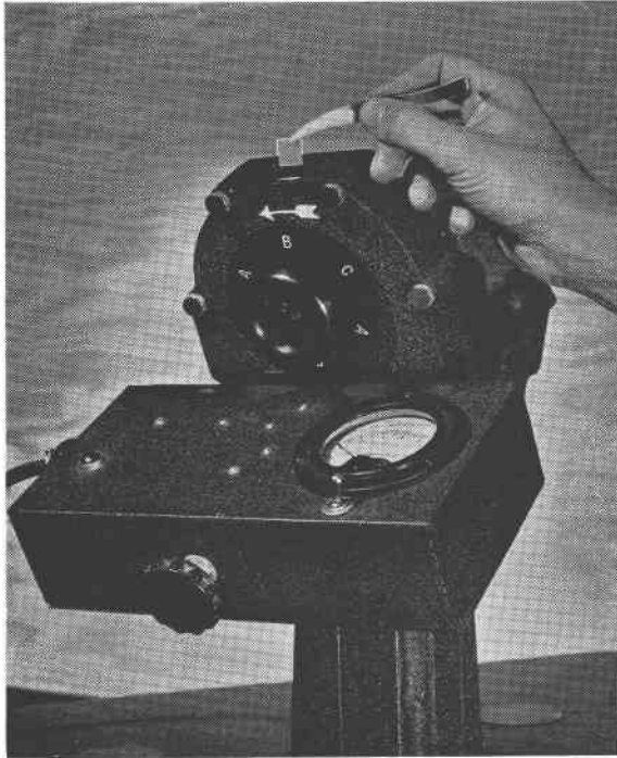
FIG. 14. Close-up view of jig used to hold and oscillate crystals during irradiation.
