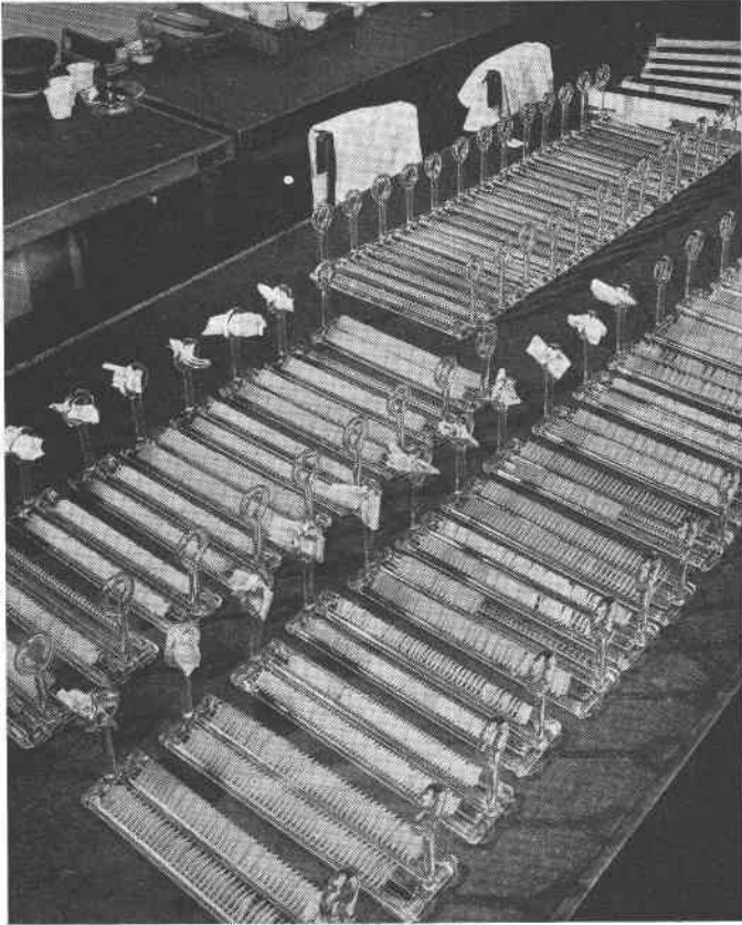
FIG. 7. Crystals racked in notched Pyrex trays, preliminary to being transferred successively to shallow tanks containing sulfuric-chromic acid cleaning solution, running rinse water, etching solution, and running water for final rinsing.
