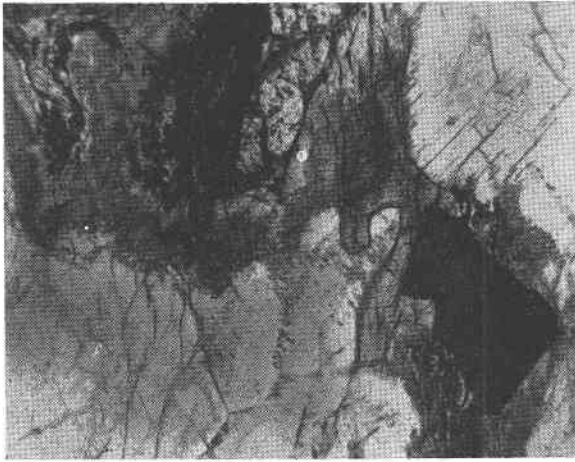
FIG. 3. C-164, plane light, \times 58 . In the upper left, olivine is surrounded by a kelyphite of greenish hornblende prisms, and is selectively replaced by iron ore. In the lower right, a corona is built about iron ore and plagioclase upon completion of replacement of olivine.
