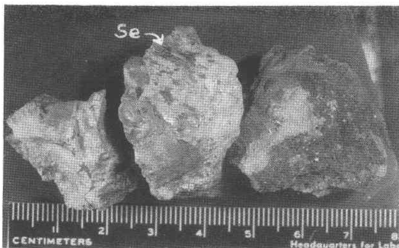
FIG. 1. Corrugated thin films of native selenium on slickensides of claystone galls in the so-called Poison Canyon sandstone, middle part of the Brushy Basin member of the Jurassic Morrison formation near Grants, New Mexico.
