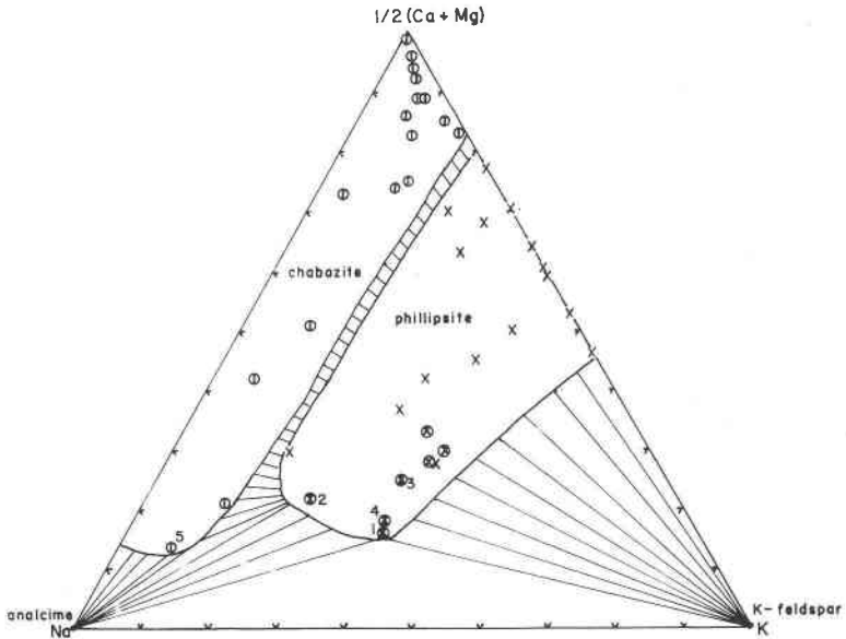
FIG. 4. \text{K-Na}-\frac{1}{2}(\text{Ca}+\text{Mg}) composition diagram for zeolites between the compositional points for analcime and K-feldspar on Fig. 3. Tie lines connect potentially co-existing minerals. Symbols for zeolite analyses as in Fig. 3. All compositional points for chabazite and phillipsite are plotted, regardless of whether or not the silica content places them in the plane of the cross-section.
