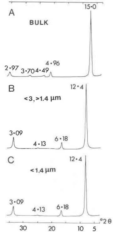
Fig. 2. X-ray diffraction patterns (maxima in Å) of air-dried sedimented aggregates of Unterrupsroth clay, \text{CoK}\alpha radiation; A = bulk sample, B = Na-saturated <3 \mu\text{m} >1.4 \mu\text{m} , C = Na-saturated <1.4 \mu\text{m} . Higher basal spacing of bulk sample (15.0Å) indicates that the clay in the natural state is saturated with divalent exchangeable cations.
