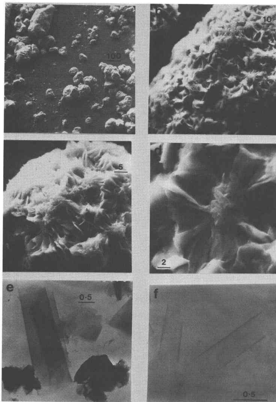
Fig. 5. Scanning electron micrographs of the Na-saturated Unterrupsroth >3.0 \mu\text{m} fraction; e and f transmission electron micrographs of the <3.0 \mu\text{m} , >1.4 \mu\text{m} and <1.4 \mu\text{m} fractions respectively. Bar scales are in \mu\text{m} .
