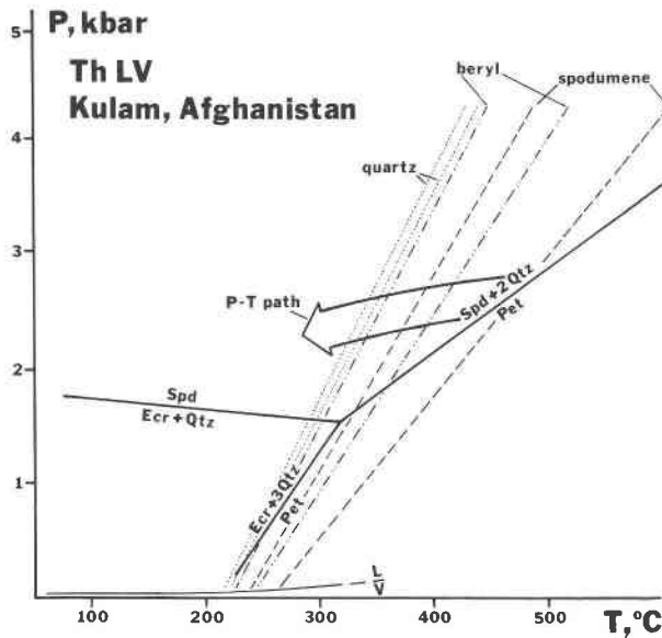
Fig. 5. Estimated conditions of pocket formation in miarolitic pegmatites of Kulam, Afghanistan (arrow), based on isochores ( T_1 , LV, partial homogenization) for spodumene and beryl constructed from microthermometric data in Fig. 3. The isochore for inclusions in quartz is derived from the microthermometric properties of the inclusions shown in Figure 4I. Phase abbreviations are eucryptite (Ecr), spodumene (Spd), petalite (Pet), quartz (Qtz), low-salinity (5 wt% NaCl) aqueous liquid (L) plus vapor (V).
