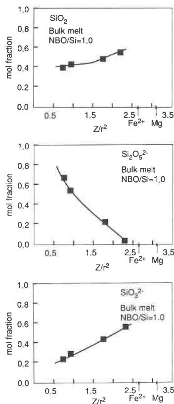
Fig. 8. Relationships between molar abundance of structural units in melts on metal oxide–silica joins and the Z/r^2 of the metal cation (data from Mysen et al., 1982a).
