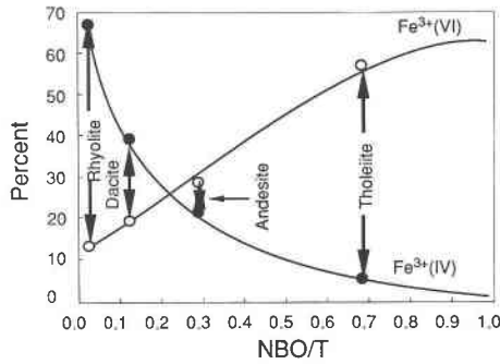
Fig. 18. Relative abundance of tetrahedrally coordinated \text{Fe}^{3+} [ \text{Fe}^{3+}(\text{IV}) ] and octahedrally coordinated \text{Fe}^{3+} [ \text{Fe}^{3+}(\text{VI}) ] in major groups of extrusive igneous rocks shown as a function of degree of polymerization of the melt. Values are calculated based on the average \text{Fe}^{3+}/\Sigma\text{Fe} (from Table 3) for the rock groups indicated (database RKNFSYS from Chayes, 1975a, 1975b, unpub. document, 1985).
