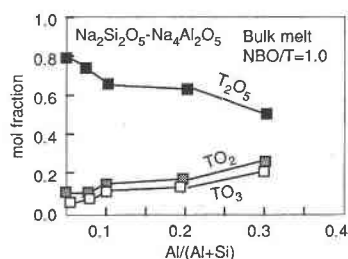
Fig. 10. Relationships between molar abundance of structural units denoted TO_2 , T_2O_5 , and TO_3 ( T = Al + Si ) as a function of Al/(Al + Si) along the sodium disilicate-sodium dialuminate join (data from Mysen et al., 1985d).
