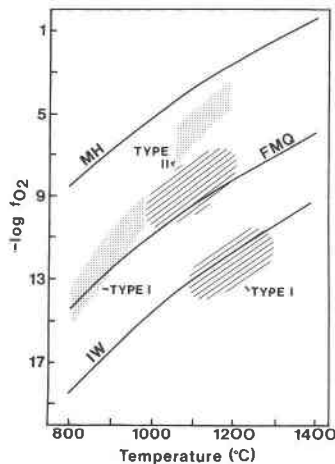
Fig. 1. Published IOF values of spinels from Cr-rich diopside group (Type I) and Al-rich augite group (Type II) spinel peridotites and ilmenite megacrysts (Arculus and Delano, 1981; Arculus et al., 1984), in hatched pattern. Thermobarometric f_{O_2} estimates (at 15 kbar) of Mattioli and Wood (1986) in shaded pattern.
