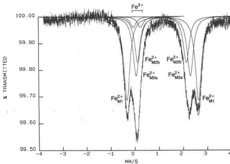
Fig. 5. The orthopyroxene separated from the Dish Hill peridotite (Ba-2-3) displays an unusually disordered Fe 2+ distribution between M1 and M2 octahedral sites. In this sample, 41% of the total Fe is Fe 2+ in the M1 site; 53% of the total Fe is Fe 2+ in the two types of M2 sites. A small amount of Fe 3+ (6% of the total Fe) is also present.
