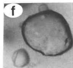
Fig. 3. Examples of extensively devitrified inclusions from the (a) Adobe Valley and (b) Mono Basin ash-flow units (inclusion 42-3) that were incompletely revitrified in the homogenization experiments at 800 °C and 2 kbar. The inclusions retained a birefringent crystalline core and crystals and vapor bubbles along the wall (c) and (d). Heating to 900 °C in a subsequent experiment resulted in (f) complete homogenization (dissolution of crystals and vapor bubbles) for the Mono Basin inclusions, but the Adobe Valley inclusion (e) remained only partially revitrified. (Larger inclusions are 120 \mu\text{m} long.)
