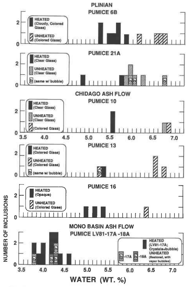
Fig. 9. Frequency diagram showing the distribution of H 2 O (as the sum of H 2 O mol + OH - as H 2 O in wt%) determined by spectroscopic analysis for unheated and heated inclusions from the same pumice samples. Pumice samples 6B, LV81-17A, and LV81-18A each consists of a single pumice clast; pumice samples 21A, 10, 13, and 16 each consists of one or more individual pumice clasts that are stratigraphically equivalent. Inclusion textures before heating are noted in figure legends and also in Tables 1 and 3. H 2 O concentrations were rounded to the nearest tenth of a weight percent for plotting as in Figure 7.
