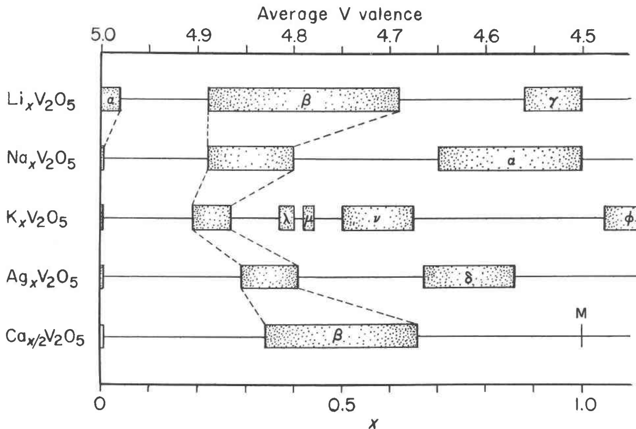
Fig. 1. Scheme showing composition ranges of various synthetic V bronzes of the type \text{M}_x\text{V}_2\text{O}_5 at about 600 °C (after Hagemmuller, 1971, 1973). The position of melanovanadite is indicated by M.
