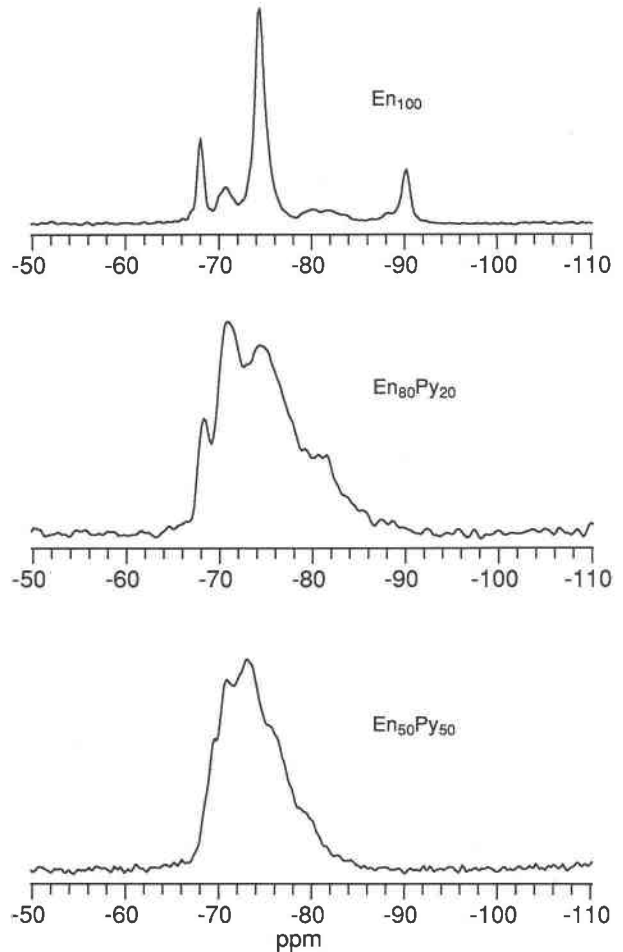
Fig. 2. Expanded 29 Si MAS NMR spectra showing the 4 Si region for En 100 , En 80 Py 20 , and En 50 Py 50 garnets. The three well-defined peaks at -68.1 ppm, -74.5 ppm, -90.2 ppm for En 100 are assigned to the T1(4Mg 0Si), T3(2Mg 2Si), and T2(0Mg 4Si) sites, respectively. The smaller, less resolved peaks are due to sites with 3Mg + 1Si and 1Mg + 3Si NNN resulting from Si,Mg disorder on the octahedral sites. Peaks for intermediate compositions are broader due to the presence of 15 possible sites as a result of Mg,Al,Si disorder on the octahedral NNN to the 4 Si.
