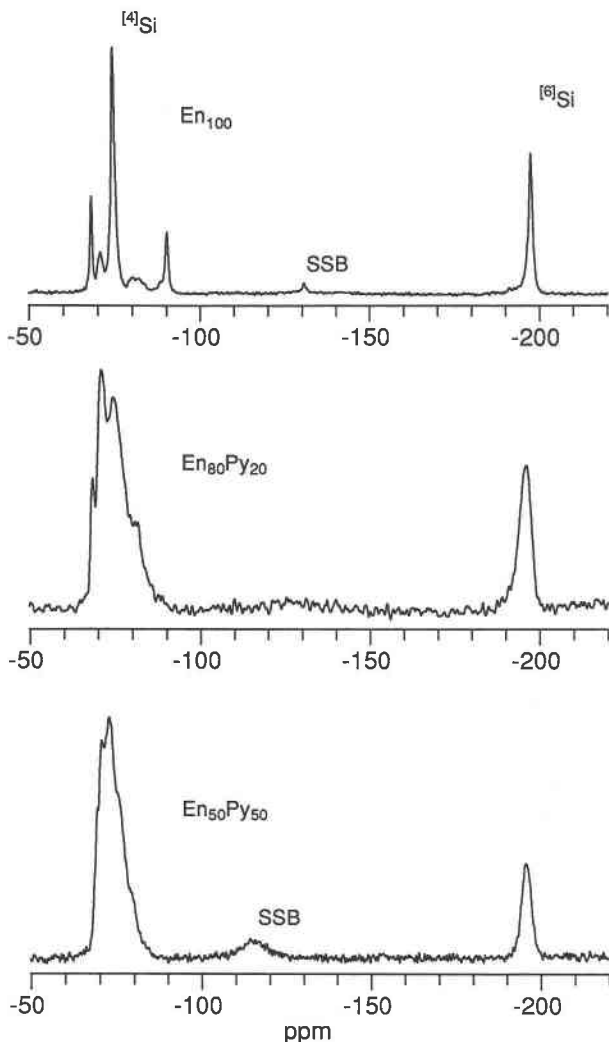
Fig. 1. The 29 Si MAS NMR spectra of En 100 , En 80 Py 20 , and En 50 Py 50 garnets, showing both 4 Si and 6 Si peaks. The chemical shifts are reported relative to tetramethylsilane (TMS).
