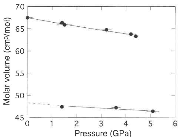
Fig. 7. Volume compression of cubanite showing the orthorhombic \rightarrow hexagonal phase transition.
