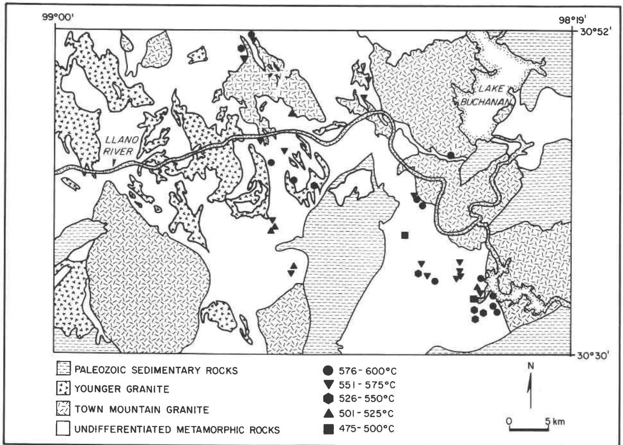
Fig. 9. Simplified geologic map of the Llano uplift showing the distribution of calcite-dolomite temperatures (see also Fig. 8). The highest temperatures are often obtained from marbles close to the granitic intrusives (see text).
