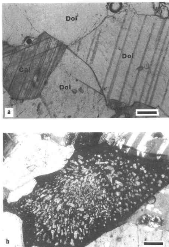
Fig. 2. (a) Photomicrograph of coexisting calcite (Cal) and dolomite (Dol) with well-developed 120^\circ triple-point junctions classified as textural type 1. (b) Photomicrograph of a calcite grain (in extinct position) containing a homogeneous distribution of exsolved dolomite. This is classified as textural type 3 (see text). Scale bar = 0.10 mm.
