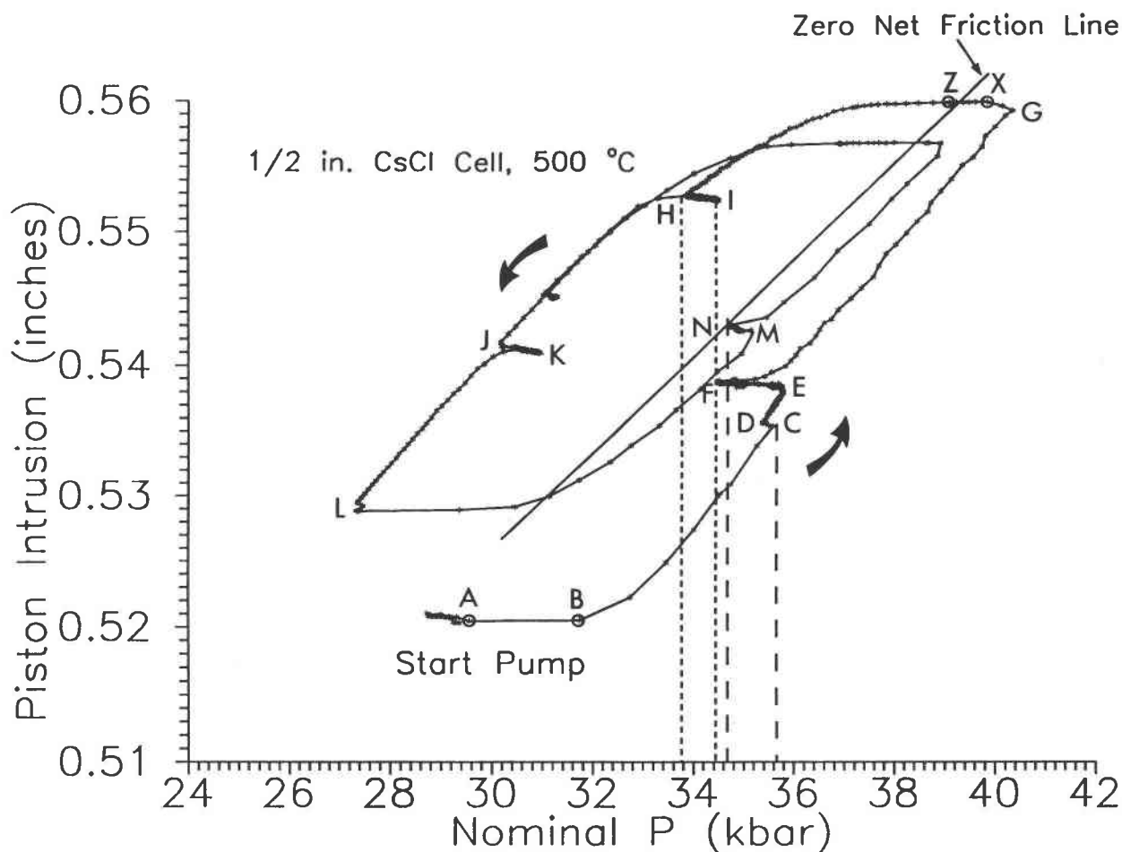
Fig. 2. Piston displacement vs. nominal pressure (hysteresis loop) of a 1/2-in. pressure cell (Fig. 1) in the piston-cylinder apparatus at 500 °C. The outer and inner loops represent first and second compression-decompression cycles, respectively.
