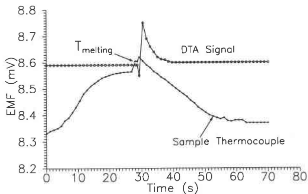
Fig. 3. Representative DTA signal due to melting of LiCl at a nominal pressure of 16 kbar, using ½-in. salt pressure cell (Fig. 1). Dots represent time of recording data in a computer.
