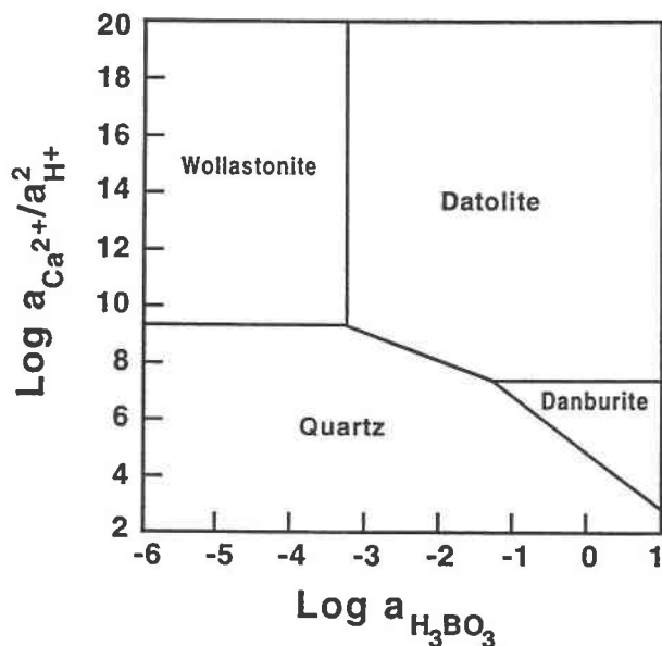
Fig. 5. Stability relations of some phases in the system CaO-B 2 O 3 -SiO 2 -H 2 O at 250 °C. SiO 2 conserved in the solid phases.
