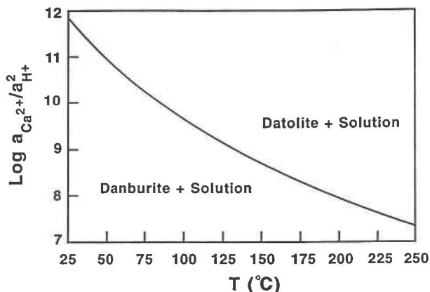
Fig. 3. Variation of the equilibrium constant ( \log a_{\text{Ca}^{2+}}/a_{\text{H}^+}^2 ) with temperature for the reaction, 2\text{CaBSiO}_4(\text{OH}) (datolite) + 2\text{H}^+ = \text{CaB}_2\text{Si}_2\text{O}_8 (danburite) + \text{Ca}^{2+} + 2\text{H}_2\text{O} . Datolite metastable below 100^\circ\text{C} .
