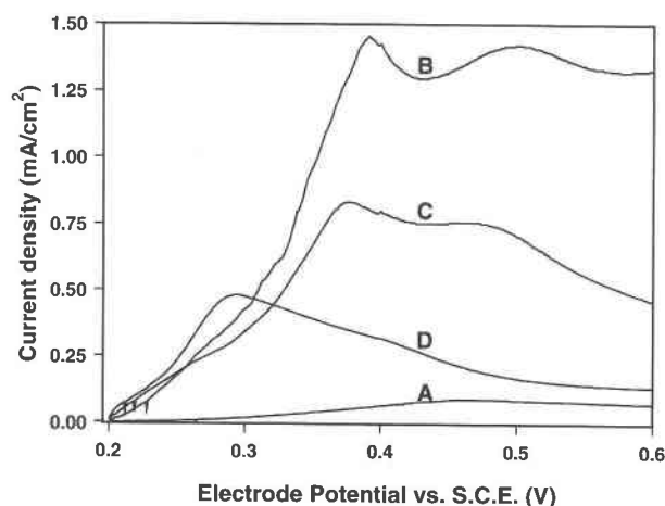
Fig. 1. Linear potential sweep voltammograms of Cu-Fe-S compounds in 1 M HClO 4 at 298 K; electrode potential sweep rate: 20 mV/s: (A) haycockite; (B) mooihoekite; (C) talnakhite; (D) chalcopyrite.
