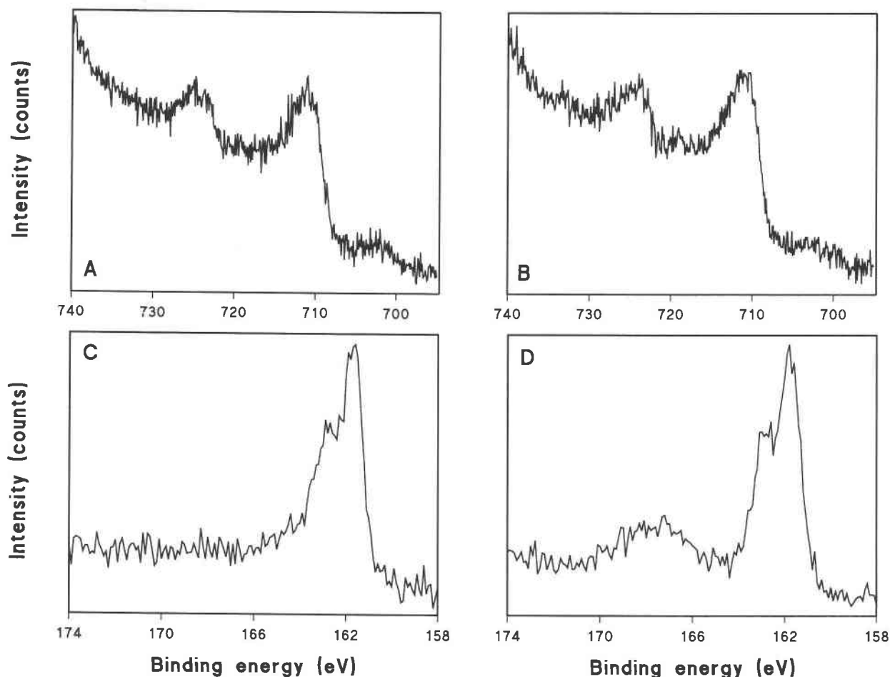
Fig. 9. XPS spectra from haycockite electrode surface oxidized in 0.1 M Na 2 B 4 O 7 at 298 K: (A) Fe 2p, oxidized at 0.1 V vs. S.C.E. with the passage of 96 C/m 2 over 170 min; (B) Fe 2p, oxidized at 0.4 V vs. S.C.E. with the passage of 92 C/m 2 over 49 min; (C) S 2p, oxidized at 0.1 V vs. S.C.E. with the passage of 96 C/m 2 over 170 min; (D) S 2p, oxidized at 0.4 V vs. S.C.E. with the passage of 92 C/m 2 over 49 min.
