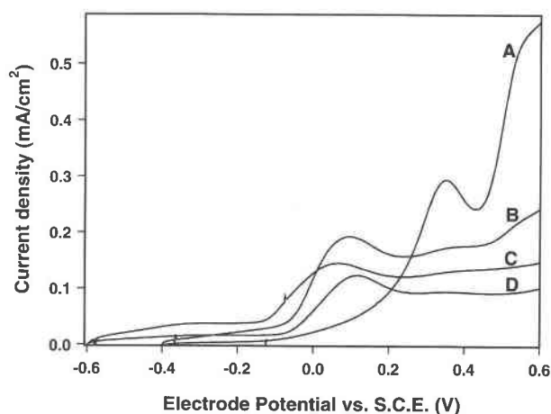
Fig. 2. Linear potential sweep voltammograms of Cu-Fe-S compounds in 0.1 M Na 2 B 4 O 7 at 298 K; electrode potential sweep rate: 20 mV/s: (A) chalcopyrite; (B) haycockite; (C) mooihoekite; (D) talnakhite.
