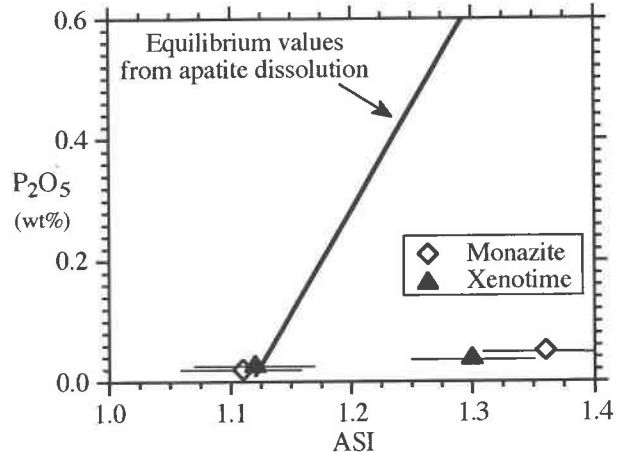
Fig. 5. Monazite and xenotime solubilities (measured as \text{P}_2\text{O}_5 in the glasses; Table 3) plotted against the Alumina Saturation Index (ASI); 750 °C, 200 \text{MPa}_{\text{H}_2\text{O}} . The line is a fit to the values of apatite solubility determined from equilibrated experiments (from Wolf and London, 1994b).
