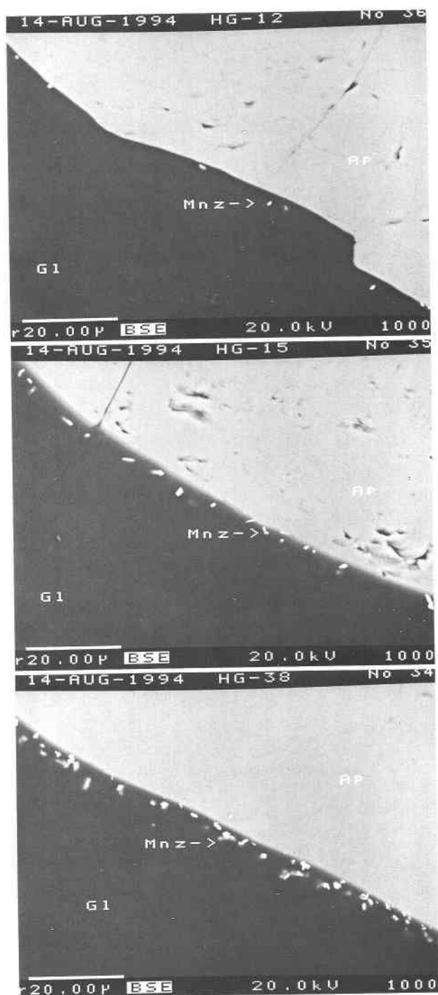
Fig. 1. Back-scattered electron (BSE) images of three Durango apatite dissolution experiments showing the increase in abundance of monazite microcrystals along the apatite-liquid interface as a function of apatite solubility, which increases with increasing Alumina Saturation Index of the liquid [ASI: mole ratio Al_2O_3/(CaO + Na_2O + K_2O) ]. Ap = apatite; Mnz = monazite; G1 = glass (quenched liquid). Scale bar in micrometers (lower left). All experiments at 750 °C and 200 MPa H 2 O . (top) No. HG-12, ASI ~1.1, 336 h, GASI.1 powder; (middle) no. HG-15, ASI ~1.2, 336 h, GASI.4 powder; (bottom) no. HG-38, ASI ~1.3, 694 h, GASI.4 powder plus additional Al 2 O 3 (see Table 1 for initial rock powder compositions).
