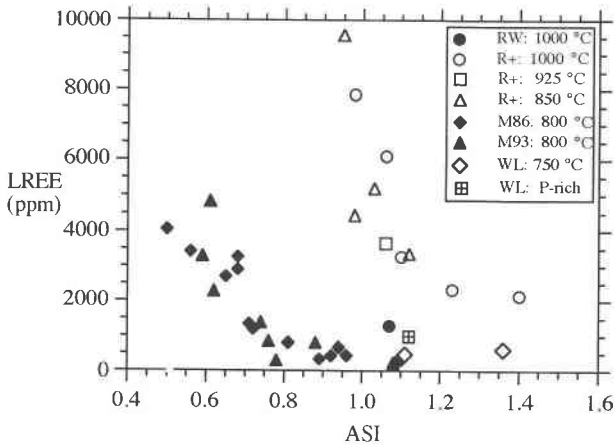
Fig. 6. Experimental monazite solubility data, as determined by total LREE content of the granitic liquids (independent of specific LREE composition), plotted against the Alumina Saturation Index (ASI) values < 1 are peralkaline, > 1 are peraluminous). Data are from Rapp and Watson (1986) = RW; Rapp et al. (1987) = R+; Montel (1986) = M86; Montel (1993) = M93; and this study = WL; P-rich sample initially contained 2.7 wt% P 2 O 5 (no. SOL-30; Table 3).
