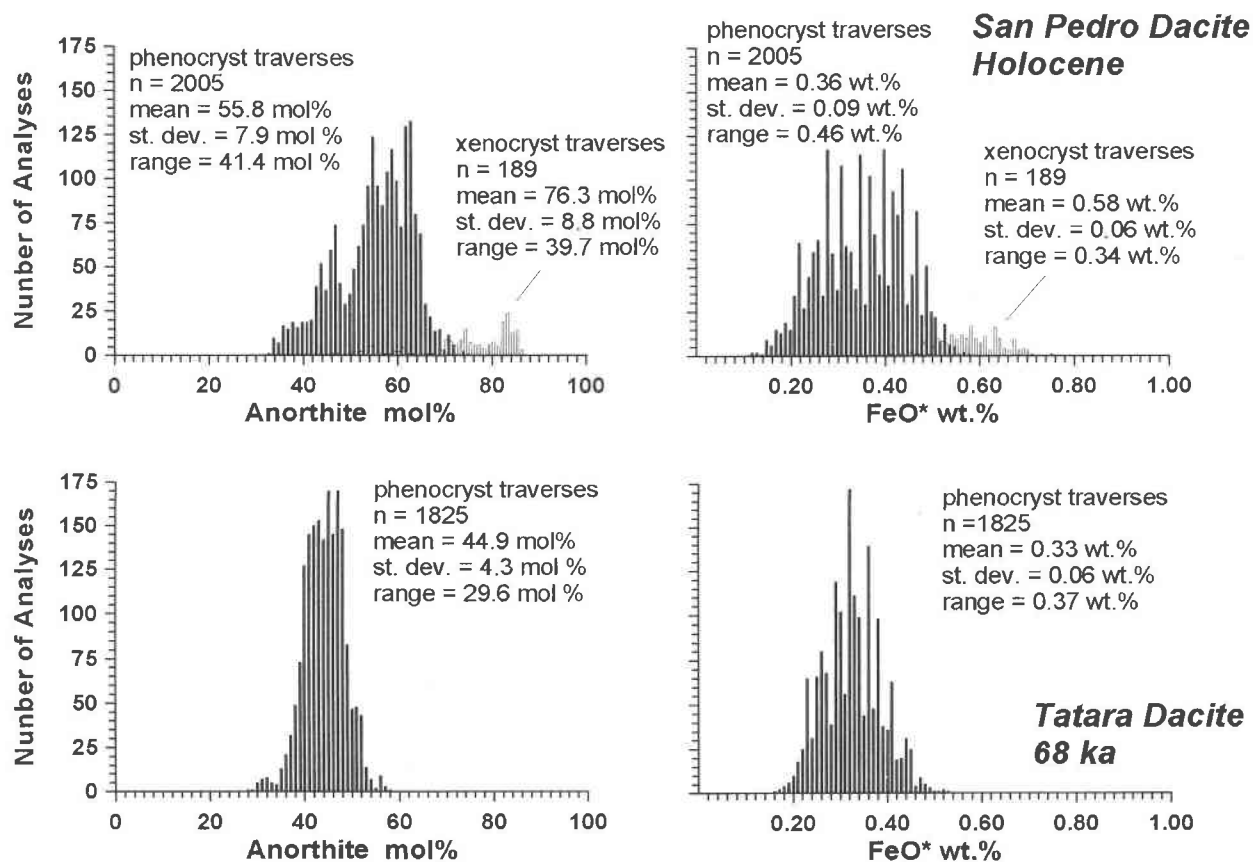
Fig. 4. Histograms summarizing >4000 EPMA measurements of plagioclase crystals in the Tataro (lower) and San Pedro (upper) dacites. Phenocrysts in dark fill, xenocrysts hollow pattern. The San Pedro dacite phenocrysts have a broader range in An content, are generally more calcic, and have higher FeO' than the Tataro phenocrysts. The San Pedro dacite contains calcic Fe-rich xenocrysts as well.
