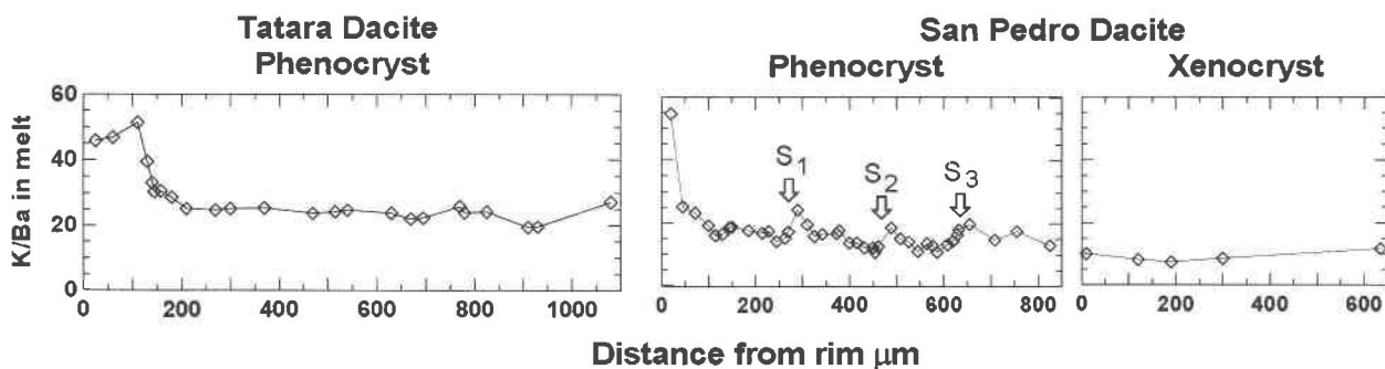
Fig. 8. Equilibrium K/Ba in melt calculated from concentrations measured in the crystals (Fig. 7). Elevated K/Ba values near the phenocryst rims record changes in the apparent partition coefficient for K owing to rapid growth. Changes in melt K/Ba recorded by oscillatory zoned intervals between major dissolution events in the San Pedro phenocryst ( S_1 , S_2 , S_3 ; Fig. 6B) imply that open-system processes repeatedly affected melts that precipitated this crystal. In this case, mixing between low K/Ba basalt, such as that which precipitated the xenocryst, and high K/Ba dacitic or rhyolitic melt is inferred.
