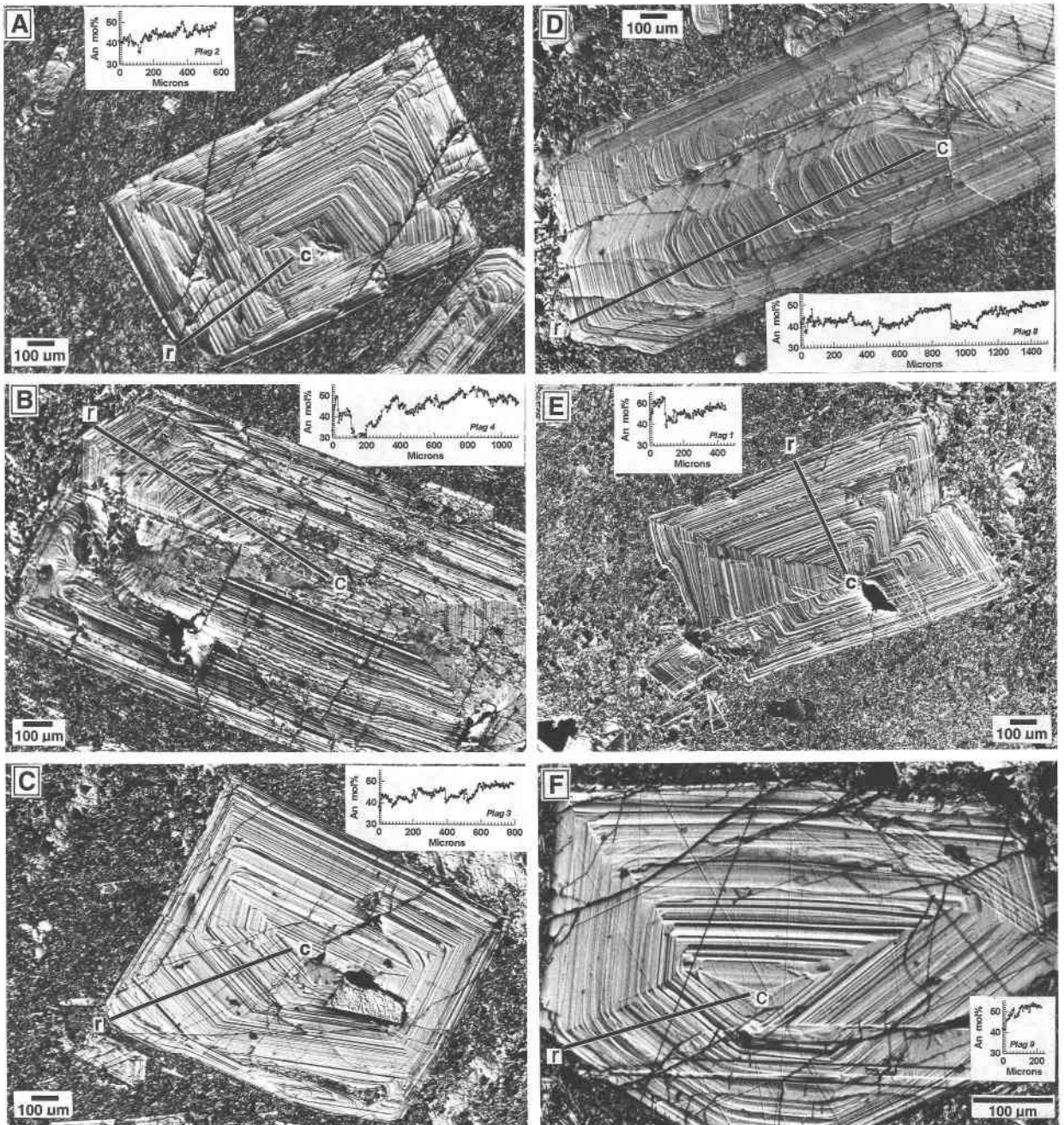
Fig. 3. NDIC images and EPMA profiles of An content vs. distance from the rim (micrometers) for six plagioclase phenocrysts in Tatara dacite sample PED-156. Note that the scale of the An profiles does not match those of the photomicrographs. Cores (c) and rims (r) of the EPMA profiles are marked on the images. In each phenocryst (A-F), many euhedral oscillatory zones are slightly truncated by several subtle dissolution surfaces. All crystals are sector zoned except in D. An profiles show small abrupt shifts at the dissolution surfaces. Within their outermost 50 \mu\text{m} , phenocrysts in A, B, C, D, and F contain intervals at reverse zoning.
