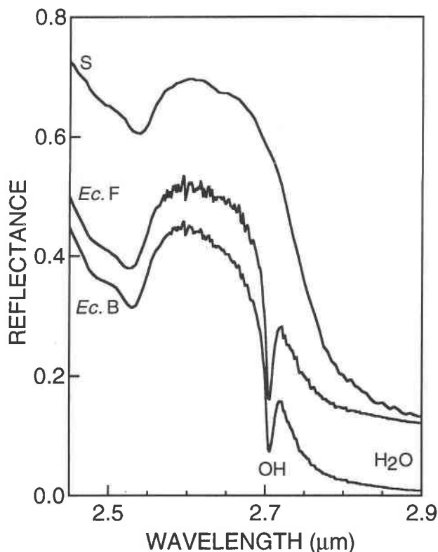
Fig. 8. OH - features in spectra of heated Echinometra spines (B) and teeth (F). Compare to the spectrum of a calcite speleothem (S), which contains features due to carbonate and H 2 O alone. The strongest brucite absorption occurs at 2.704 μm, whereas portlandite produces one at 2.744 μm (Ryskin, 1974). The position of the OH - feature in spectra of heated echinoid samples is similar to that of brucite. Noise in the 2.6 μm region in the echinoid spectra is due to variations in atmospheric H 2 O in the path of the spectrometer beam. The positions of carbonate bands in this spectral region are a function of cation mass (Gaffey, 1987). The 2.5 μm carbonate feature occurs at shorter wavelengths in echinoid spectra than in the speleothem spectrum because of the Mg content of the former. Spectra offset vertically for comparison. Ec. = Echinometra .
