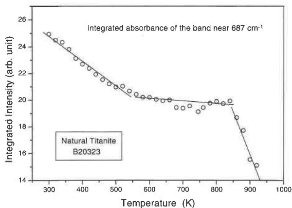
FIGURE 7. The integrated intensity of the 687 cm -1 band in sample B20323 shown as a function of temperature. For integration, a linear baseline between the spectral minima on either side of the peaks was used. The change in temperature dependence between 500 and 600 K corresponds to the phase transition at 500 K for the synthetic titanite sample (Bismayer et al. 1992; Salje et al. 1993; Zhang et al. 1995). The lines are visual guides.
