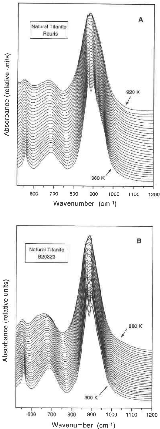
FIGURE 2. Temperature evolution of the IR spectra of titanite samples (A) Rauris and (B) B20323 between 500 and 1200 \text{cm}^{-1} . The temperature interval is 20 K.
