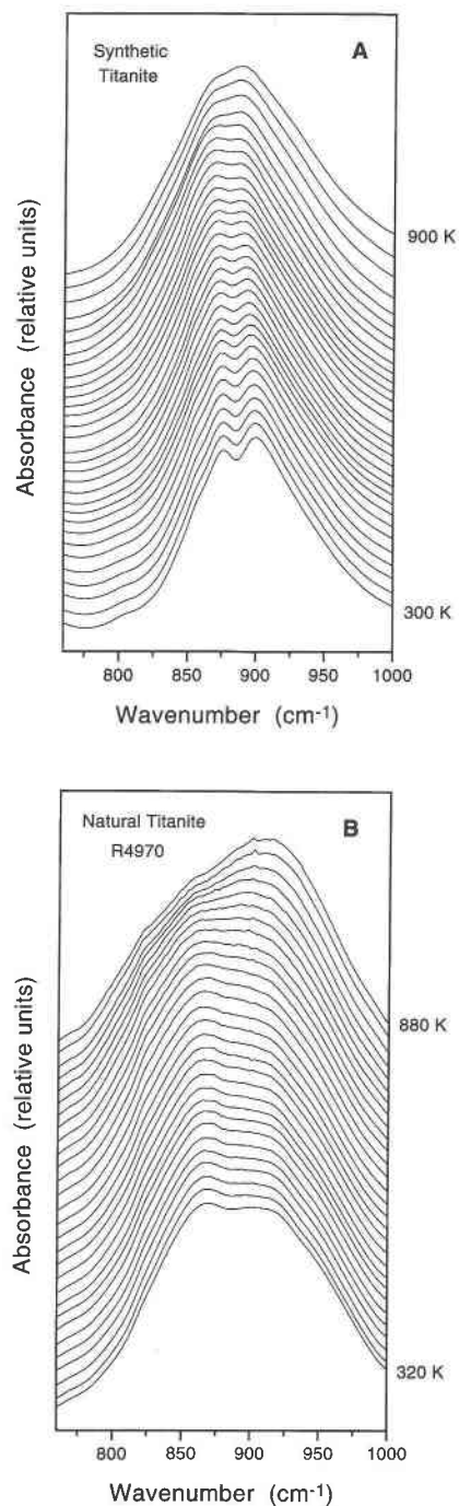
FIGURE 3. Stack plot of the IR spectra of (A) synthetic titanite and (B) sample R4970 between 720 and 1000 \text{cm}^{-1} , showing details of the spectral changes during the structural phase transition. The temperature interval is 20 K.
