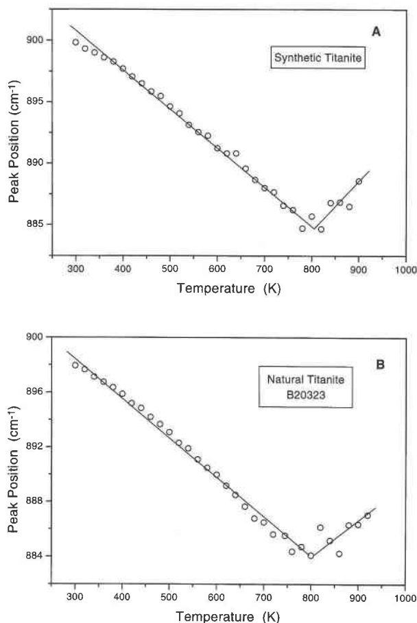
FIGURE 5. The temperature evolution of the Si-O stretching band near 899 cm -1 . (A) Synthetic sample; (B) B20323.
