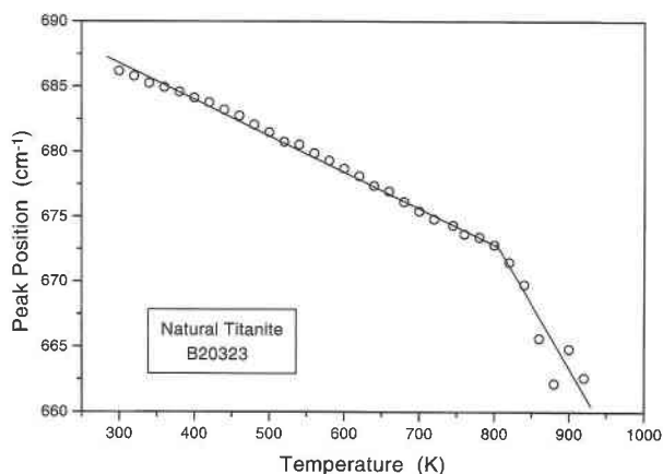
FIGURE 6. The IR band near 685 cm -1 of sample B20323 shows strong phonon softening at temperatures above 825 K.
