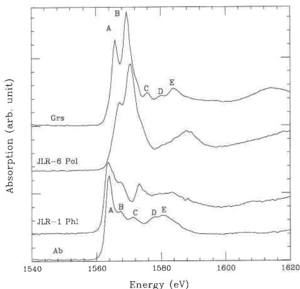
FIGURE 3. Experimental XANES spectra at the Al K edge of reference the minerals grossular (Grs) and albite (Ab) and of two synthetic micas containing either ^{61}\text{Al} only (polyolithionite, JLR-6) or ^{27}\text{Al} only (phlogopite, JLR-1). See text for explanation of peak labels.
