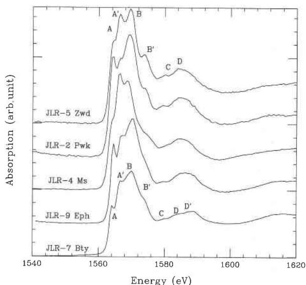
FIGURE 4. Experimental XANES spectra at the Al K edge of synthetic micas containing Al in two types of coordination. From top to bottom: zinnwaldite (JLR-5), preiswerkite (JLR-2), muscovite (JLR-4), ephesite (JLR-9), and bityite (JLR-7).
