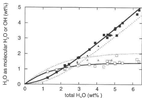
FIGURE 3. H 2 O speciation as a function of total H 2 O content. Open and closed symbols indicate hydroxyl and molecular H 2 O, respectively; squares are phonolite data (this study), triangles are jadeite data (Silver et al. 1990). Solid curves are model speciation for phonolitic glass, on the basis of fit of data to Equation 4 as described in text. Dashed curves show Dixon et al. (1995) model speciation data for hydrous basaltic glass quenched from 1200 °C.
