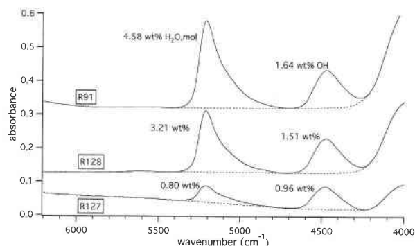
FIGURE 1. Representative FTIR spectra of three phonolitic glasses with 1.76, 4.72, and 6.22 wt% total dissolved H 2 O; see Table 2 for synthesis conditions. Approximate backgrounds are indicated with dashed lines, and numbers next to peaks are calculated quantities of molecular H 2 O (5200 cm -1 ; \epsilon_{5200} = 1.10 ) and hydroxyl (4500 cm -1 ; \epsilon_{4500} = 1.25 ). Spectra have been normalized to a 400 \mu m sample thickness.
