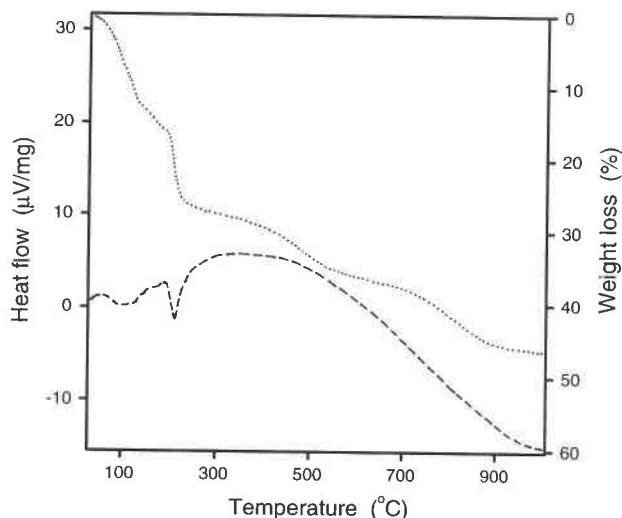
FIGURE 3. Thermogravimetric (dotted line) and heat flow (dashed line) curves measured on 1.68 mg of powdered gordaite from Hettstedt.
