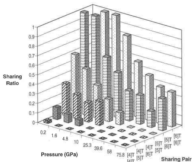
FIGURE 4. Calculated sharing ratios for selected \text{TO}_n polyhedra as a function of pressure. The sharing ratio for a given polyhedra pair (e.g., ^{6}\text{T} - ^{6}\text{T} ) is defined as the ratio of the number of \text{TO}_6 - \text{TO}_6 pairs that corner share to the number of \text{TO}_6 - \text{TO}_6 pairs that edge share. The propensity of edge sharing in any polyhedra pair involving at least one \text{TO}_6 subunit is clearly seen as is the ability of \text{TO}_5 polyhedra to actively take part in corner sharing preferentially with \text{TO}_4 and edge-sharing with \text{TO}_6 .
