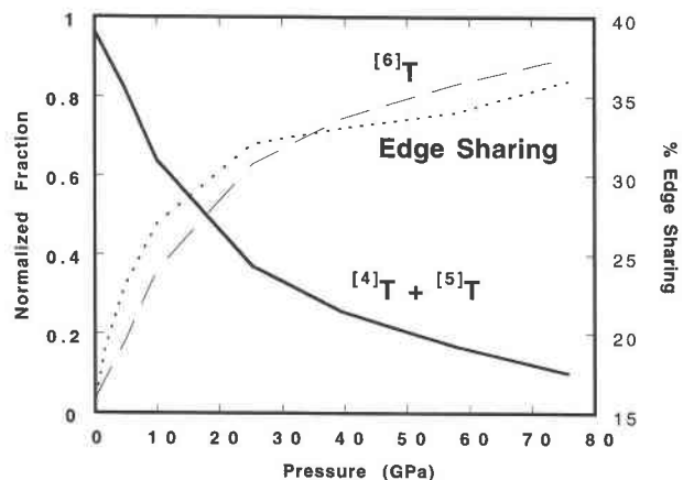
FIGURE 3. The calculated number fraction abundance of ^{6}\text{T} (dashed curve) and ^{4}\text{T} + ^{5}\text{T} (solid curve) normalized to unity and plotted against pressure at 4000 K for \text{CaAl}_2\text{Si}_2\text{O}_8 . Dotted curve, the number fraction of edge-sharing \text{TO}_n polyhedra. The correlation of the fraction of polyhedra that take part in edge sharing with abundance of ^{6}\text{T} is consistent with the distribution of T-O-T angles in Figure 2.
