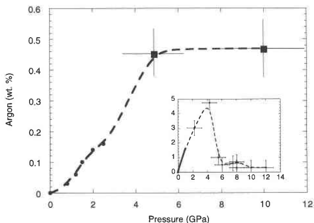
FIGURE 6. Solubility of Ar in molten anorthite from White et al (1989), shown by the solid circles, and Chamorro-Perez et al (1996), shown by the solid squares, at approximately 2000 K as a function of pressure. The pressure dependence of the solubility approaches zero in the same pressure interval that the \text{TO}_4 -based ring structure is destroyed as edge-sharing \text{TO}_5 and \text{TO}_6 polyhedra dominate the system. Inset shows solubility relations in molten silica from Carroll and Stolper (1991) for comparison. This figure is modified from Figures 4 and 7 in Chamorro-Perez et al (1996).
