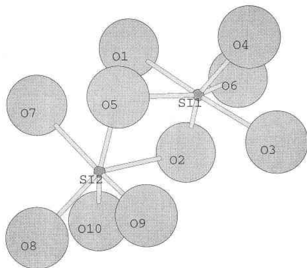
FIGURE 5. Oblique view of a pair of edge-sharing ^{16}\text{T} from an MD simulation at 25.3 GPa and 4000 K. The O-T-O angle \text{O}_5\text{-Si}_1\text{-O}_2 is 89.4^\circ and the O-T-O angle \text{O}_5\text{-Si}_2\text{-O}_2 is 73.7^\circ . The Si-O-Si angle is either 101^\circ ( \text{Si}_1\text{-O}_5\text{-Si}_2 ) or 92.2^\circ ( \text{Si}_1\text{-O}_2\text{-Si}_2 ). The ions O2, O4, O5, O6, O8, and O10 are approximately coplanar.
