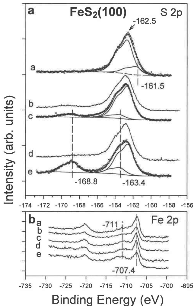
FIGURE 2. S 2p (top) and Fe 2p (bottom) data of FeS 2 (100) after (a) acid-washing, (b) exposure to 20 h of H 2 O vapor, (c) 400 h of H 2 O vapor, (d) 20 h of O 2 , and (e) 20 h of a H 2 O vapor/O 2 mixture.
