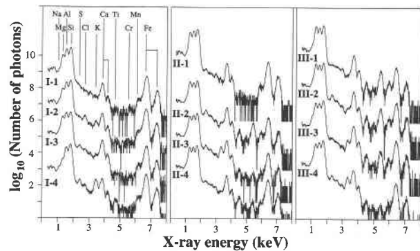
FIGURE 3. PIXE (0.65 MeV protons) spectra collected for garnets cloisonnés as compared to garnets standards. Left: PIXE spectra for type I garnets. I-1 = cloisonné no. 8 in LM1; I-2 = cloisonné no. 3 in LM 41; I-3 = eclogitic Mg-almandine from Petzthal, Austria; I-4 = almandine from Zillertaler, Austria. Middle: PIXE spectra for type II garnets: II-1 = analysis no. 1 in LM57; II-2 = Cr-pyrope from Merofritz, Bohemia, Czech Republic; II-3 = charnockitic pyrope from Arendal, Norway; II-4 = eclogitic pyrope from Kimberley, R.S.A. Right: PIXE spectra for type III garnets: III-1 = cloisonné no. 12 in LM3; III-2 = Cr-pyrope from Podsedice, Bohemia, Czech Republic; III-3 = Cr-rich pyrope from Zöblitz, Saxony, Germany; III-4 = eclogitic pyrope from Monastir, R.S.A.
