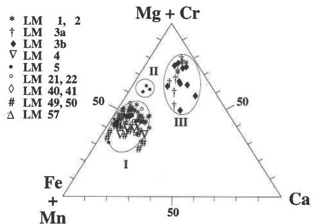
FIGURE 4. Ternary diagram for garnet cloisonnés compositions measured on Louvres artifacts showing the three types of garnet composition.
