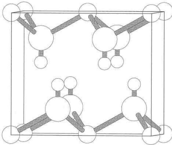
FIGURE 1. The structure of brucite. Big ball represents O, medium ball represents Mg, and small ball represents H.
