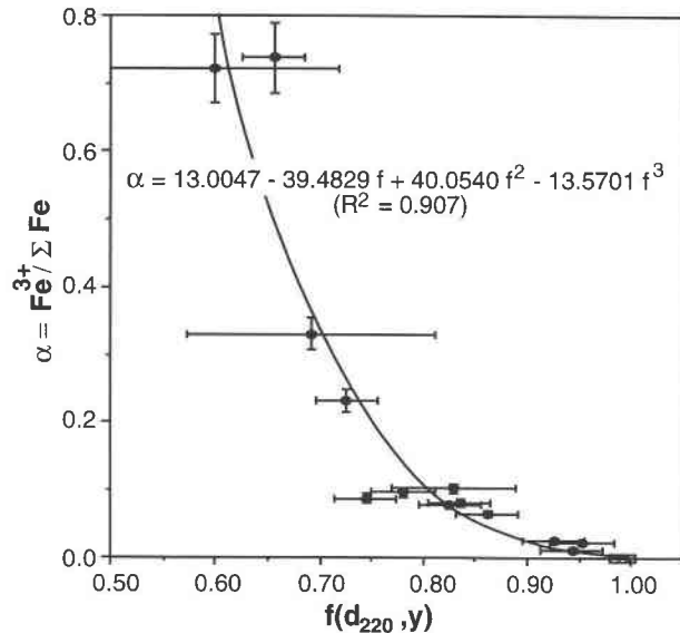
FIGURE 2. The effect of non-stoichiometry on d_{220} : f_{obs} = (d_{220(\alpha)} - 1.498)/(d_{220(0)} - 1.498) . Solid circles are for samples equilibrated at various oxygen fugacities; open squares for nominally stoichiometric magnesiowüstite equilibrated at C-CO.
