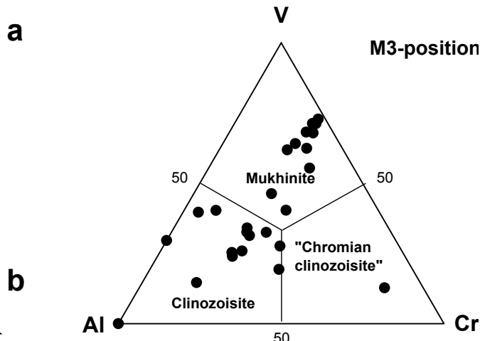
FIGURE 7. Ternary V-Al-Cr diagram of epidote group minerals from C-rich amphibole schists of the PPCC.
