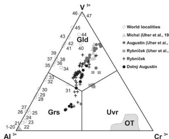
FIGURE 3. Ternary V-Al-Cr diagram (atomic proportions) of garnet from C-rich amphibole schists of the PPCC in comparison to the world occurrences (1 to 47, for locality explanations see Uher et al. 1994). Abbreviations of compositional fields: OG = Ogcheon belt, Korea (Jeong and Kim 1999); PB = Poblet area, Spain (Canet et al. 2003); OT = V-bearing uvarovite from Outolumpu, Finland (von Knorring et al. 1986).
