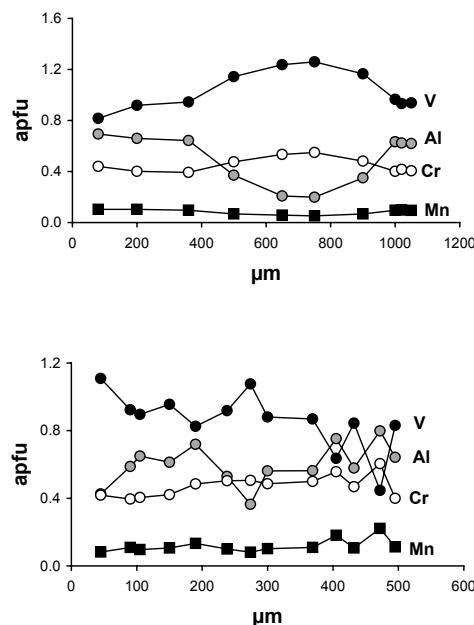
FIGURE 4. Compositional profiles through garnet crystals from C-rich amphibole schists of the PPCC.
