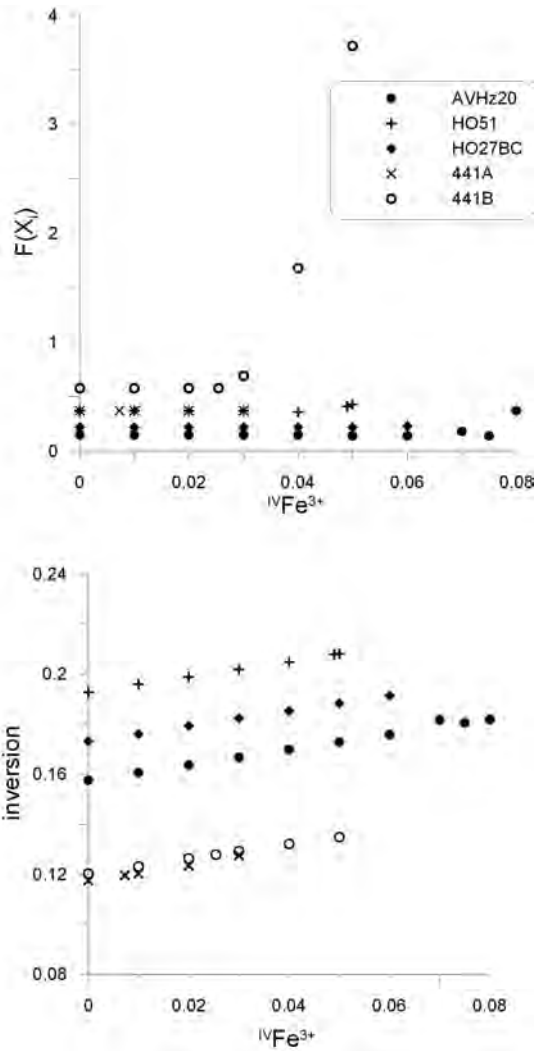
FIGURE 2. Plot of the minimization function (a) and of the inversion parameter (b) obtained by optimizing the distribution of Mg, Al, and \text{Fe}^{2+} with \text{IVFe}^{3+} fixed at the values in abscissa. The minimization function does not change significantly over a wide range of \text{IVFe}^{3+} , the only exception is 441B hercynite, which seems to preclude complete tetrahedral \text{Fe}^{3+} ordering.
