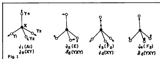
Fig. 1. Forms of vibration for the (\text{AsO}_4)^{3-} tetrahedral group.
