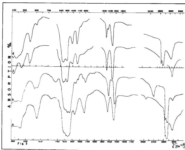
Fig. 3. Infrared spectra of conicalcite and austinite: (a) conicalcite from Lachin-han, USSR; (b) deuterated conicalcite from Lachin-han; (c) austinite from Hovon-aksi, USSR; (d) austinite from Ojue'a, Mexico. For \text{cm}^{-17} read \text{cm}^{-1} .
