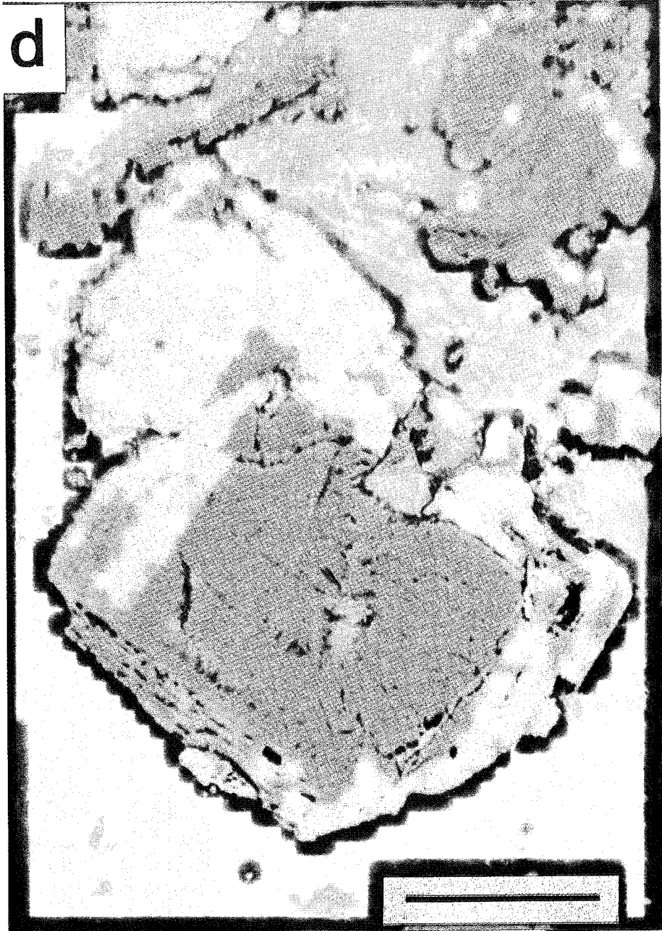
FIG. 3d. Optical micrograph of stained arsenopyrite grain from Fairview mine showing color contrast. Scale bar is 0.1 mm.
