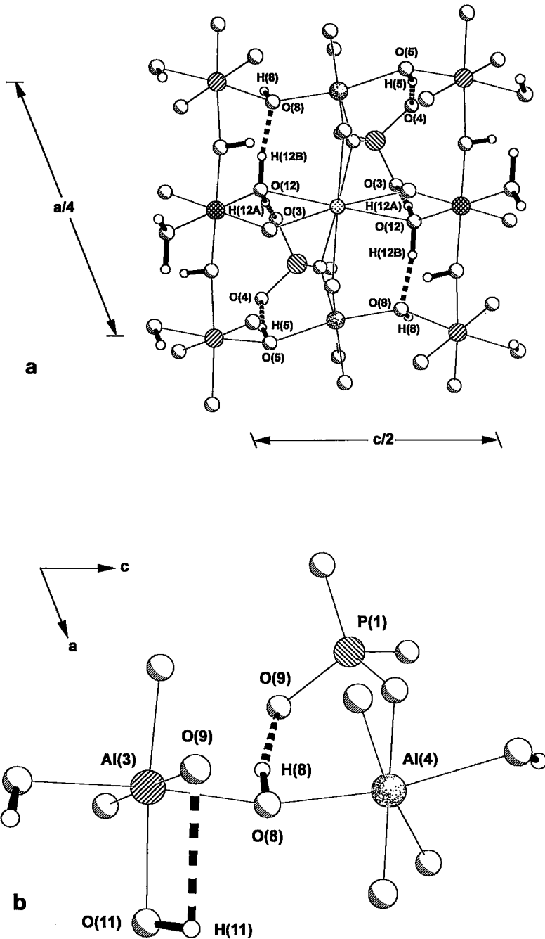
FIG. 4. Hydrogen bond in the structure of burangaite projected onto (010): (a) hydrogen bonding for H(5), H(12A) and H(12B), and (b) hydrogen bonding for H(8) and H(11). D-H and H...A bonds (D: donor, A: acceptor) are given as heavy full and broken lines, respectively. Al(3) cations have bottom left to top right parallel-line shading, Al(4) cations have heavy random-dot shading, P(1) and P(2) cations have bottom right to top left parallel-line shading, Al(1) cations have hatched shading, and Na cation has regular-dot shading.
