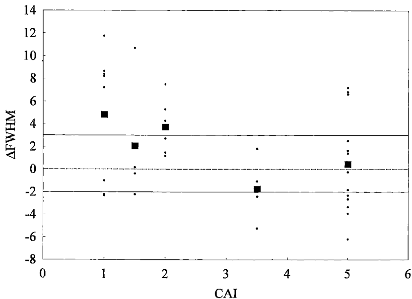
FIG. 7. Change in emission bandwidth ( \Delta FWHM ) induced by heating plotted against CAI. Mean values for each CAI group are shown as large filled symbols. The lines at -2 and +3 nm enclose the data from synthetic calcite (Mason 1994; unpubl. data).
