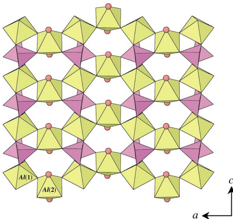
FIG. 1. Ordered part of the crystal structure of nevadaite, projected onto (010); (Alφ 6 ) octahedra are shaded yellow, (PO 4 ) tetrahedra are shaded pink, (H 2 O) groups are shaded red circles. Note the decorated [Alφ 5 ] corner-sharing chains that extend along a and link by sharing octahedron–tetrahedron vertices along c .
