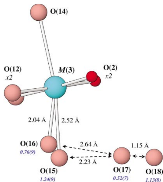
FIG. 4. Local configuration associated with the two positionally split ( \text{H}_2\text{O} ) groups, O(15)–O(16) and O(17)–O(18). Legend as in Figure 3; smaller darker red circles are \text{O}^{2-} . The interatomic distances are indicated with dashed lines, and site occupancies are given in purple text.
