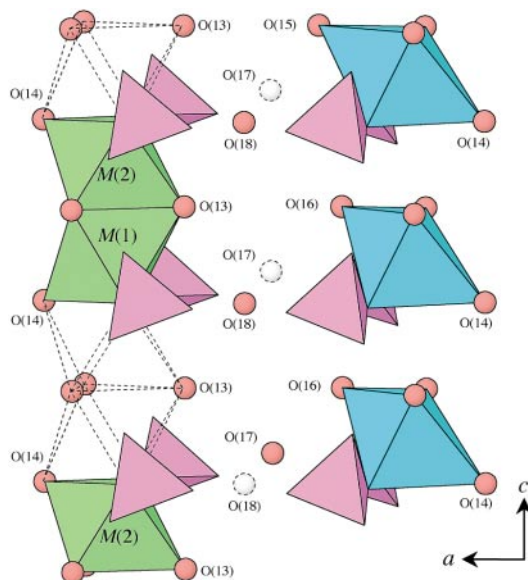
FIG. 5. Example of a locally ordered arrangement within the disordered layer; legend as in Figures 3 and 4.
