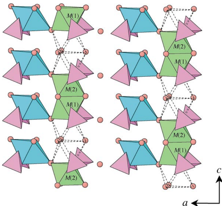
FIG. 2. Disordered part of the crystal structure of nevadaite, projected down an axis 8^\circ from [010] ; occupied M(1) and M(2) octahedra are shaded green, unoccupied M(1) and M(2) octahedra are outlined by dashed lines, and M(3) octahedra are shaded blue. The (H_2O) groups at O(16) and O(17) are not shown.
