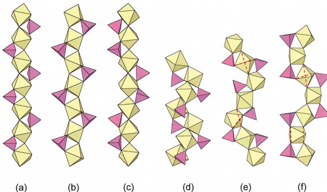
FIG. 7. [M(TO_4)\phi_3] chains in selected mineral structures: (a) butlerite, (b) metavauxite, (c) stewartite, (d) fibroferrite, (e) slavikite, and (f) nevadaite.
