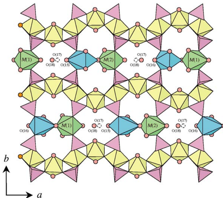
FIG. 3. The crystal structure of nevadaite projected onto (001); legend as in Figures 2 and 3. Note that the disordered layers are shown in an arbitrarily ordered fashion. Vacant O(17) and O(18) sites are shown with dashed circles.
