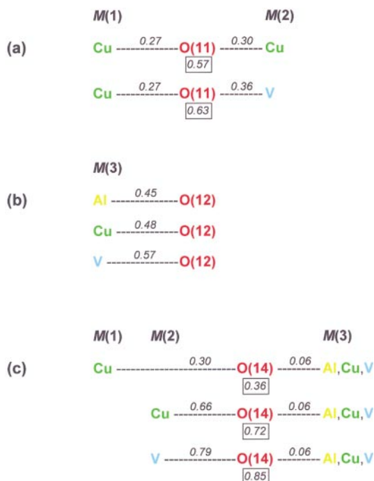
FIG. 6. Bond valences associated with Cu, V and Al at the M sites for (a) O(11), (b) O(12), and (c) O(14).
