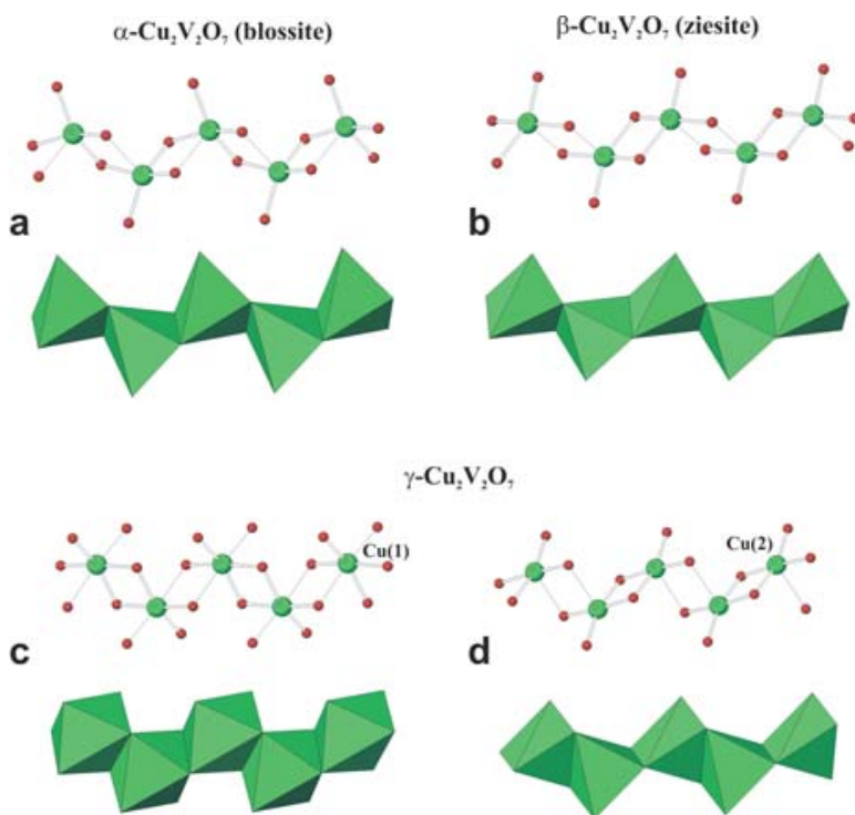
FIG. 2. Chains of Cu coordination polyhedra in the structures of blossite (a), ziesite (b) and \gamma\text{-Cu}_2V_2O_7 (c, d). Legend: \text{Cu}^{2+} cations: green, \text{O}^{2-} anions: red, \text{Cu}^{2+} coordination polyhedra: green.
