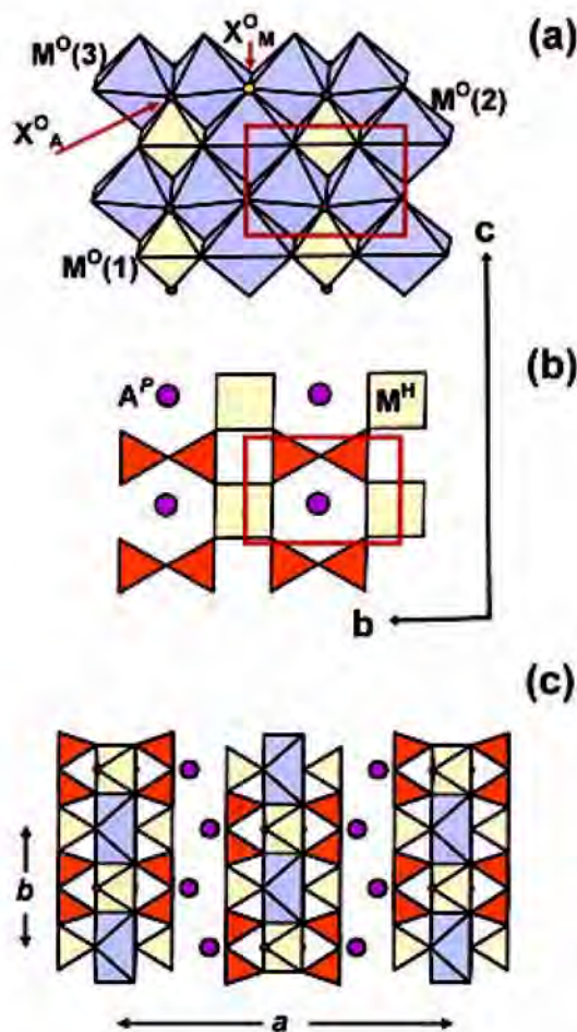
FIG. 1. The crystal structure of barytolampoptyllite: the O sheet (a) and the H sheet (b) of the TS block as viewed down [100] ; general view of the crystal structure projected onto (001) (c). (SiO_4) tetrahedra are orange, Na octahedra are navy blue, Ti polyhedra, [5]M^H and [6]M^O(1) , are yellow, the A^P atoms are shown as raspberry circles, the planar cell with translations t_1 \approx 5.5 Å and t_2 \approx 7 Å is shown in red.
