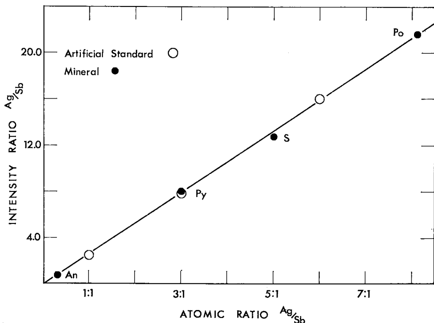
FIG. 3. Standardization Curve for Ag/Sb.
