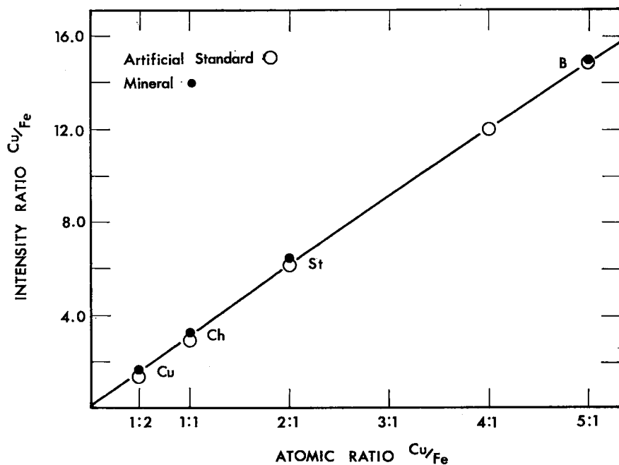
FIG. 1. Standardization Curve for Cu/Fe.
