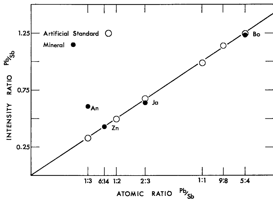
FIG. 2. Standardization Curve for Pb/Sb.
