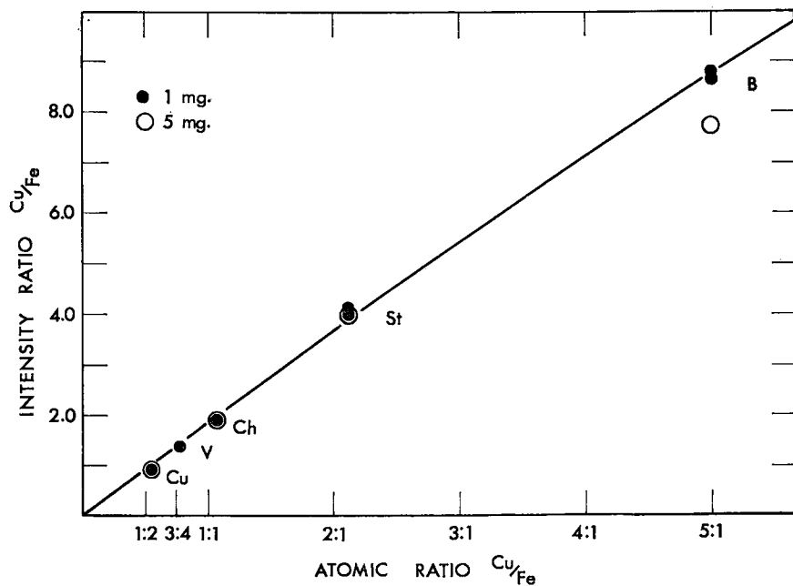
FIG. 5. Working Curve for Cu/Fe.
