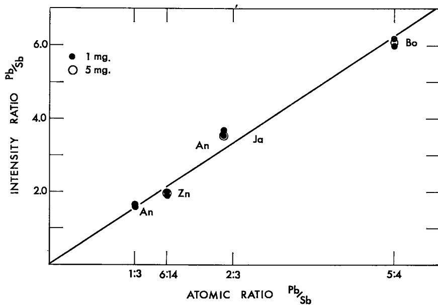
FIG. 6. Working Curve for Pb/Sb.
