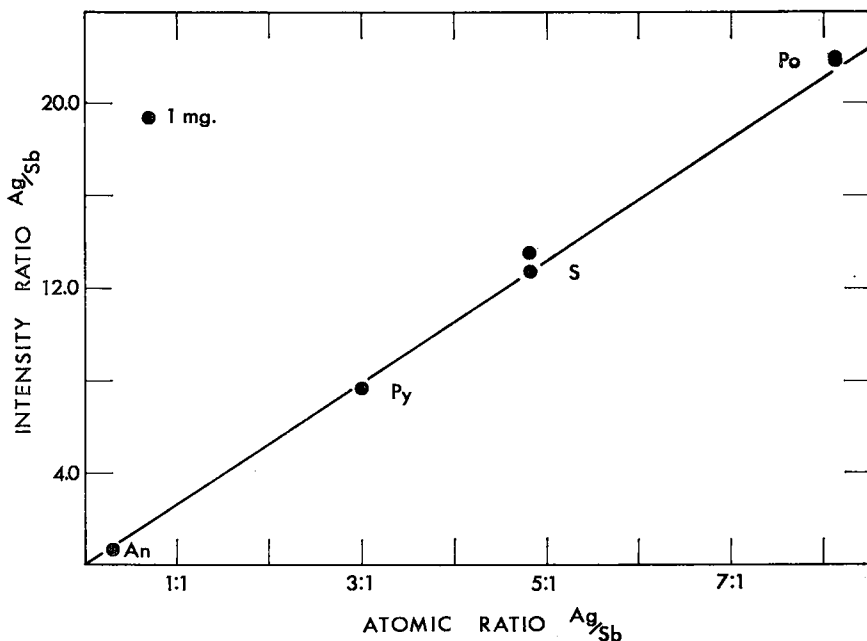
FIG. 7. Working Curve for Ag/Sb.
