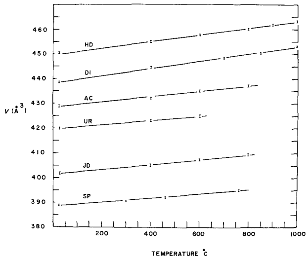
FIG. 6. Variation of unit cell volume with increasing temperature for six clinopyroxenes. (Abbreviations are the same as those in Figure 2.) Error bars represent \pm 1 standard deviation.
