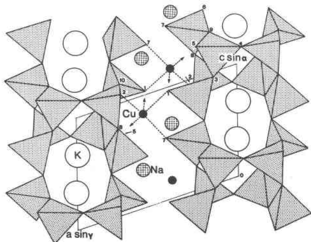
FIG. 1. The crystal structure of litidionite projected along [010]. The bonds terminated by an arrow refer to oxygen atoms O(1) and O(5) occurring in chains which are not shown in the figure.
