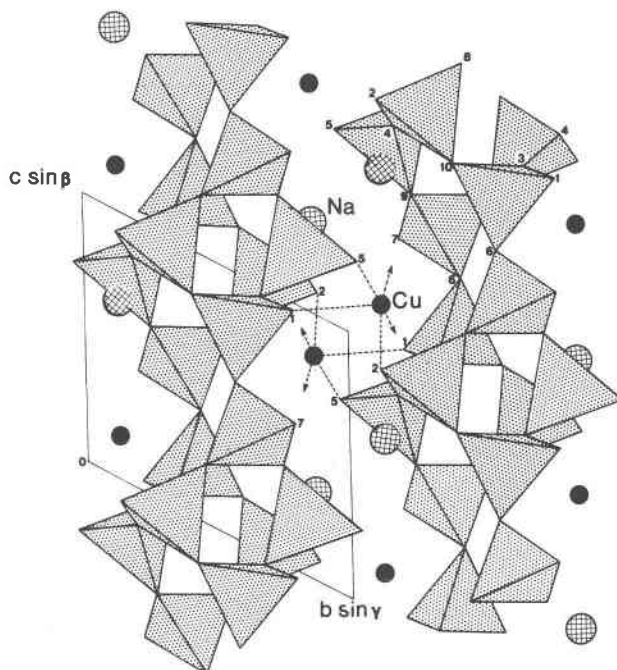
FIG. 2. The crystal structure of litidionite projected along [100]. The bonds terminated by an arrow refer to oxygen atoms O(1) and O(7) occurring in chains which are not shown in the figure. The potassium atoms have been omitted for clarity.
